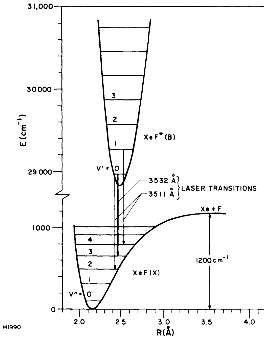
Figure 14 XeF Lasing Transitions
