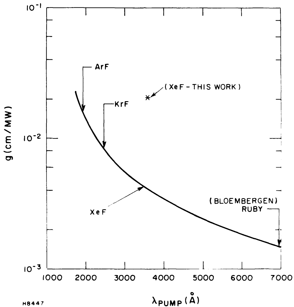
Figure 13 First Stokes Gain for Forward SRS in H_2 . Solid line is wavelength-scaled calculation normalized to Bloembergen's result with ruby; * indicates the value deduced from this work.
