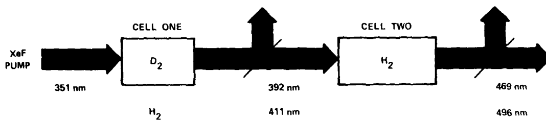
Figure 6 Two-step two-cell Raman conversion to the Blue/Green.
