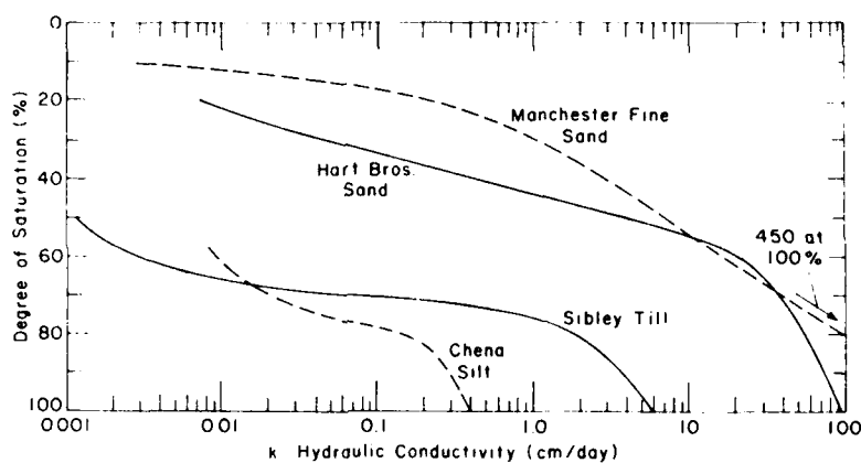
Figure 6. Hydraulic conductivity vs degree of saturation.
