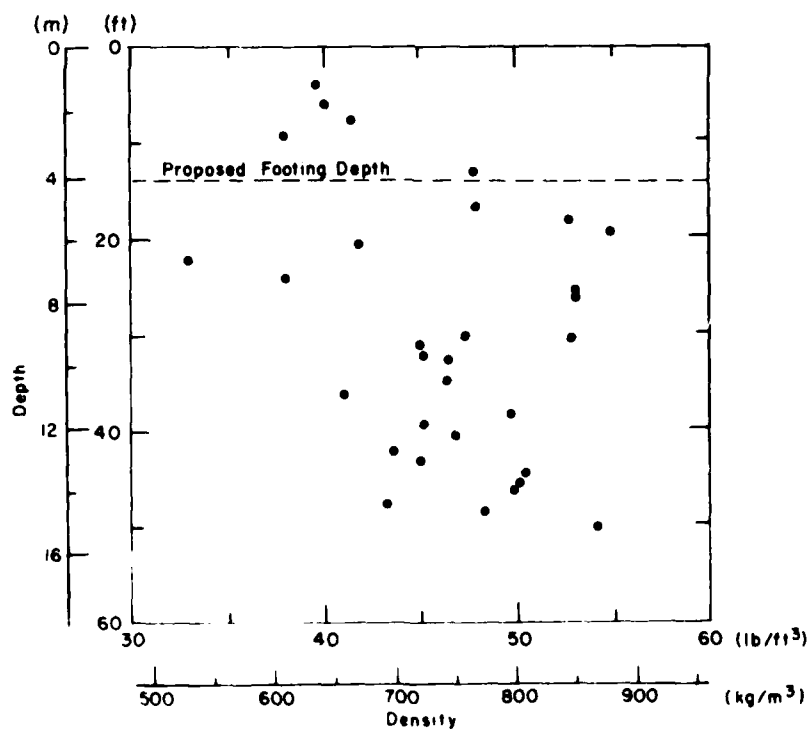
b. Density vs depth.
