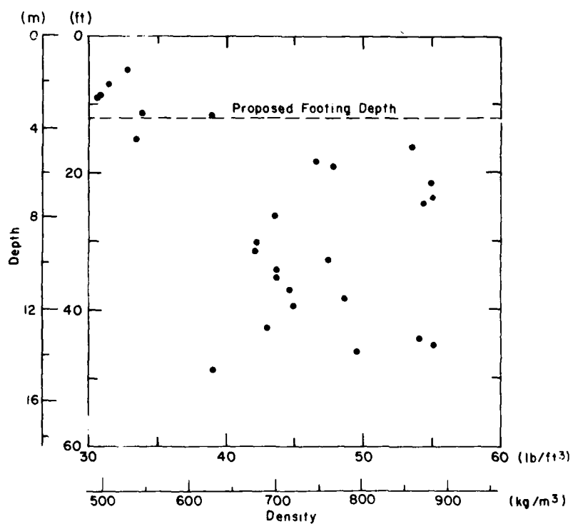
b. Density vs depth.
