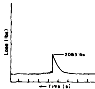
Figure B11 Sample E22 (time interval 1s)
