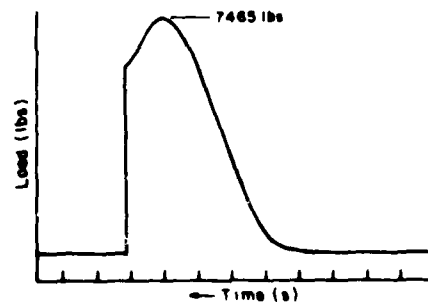
Figure B12 Sample E39 (time interval 1s)
