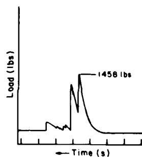
Figure B2. Sample A23 (time interval 1s).
