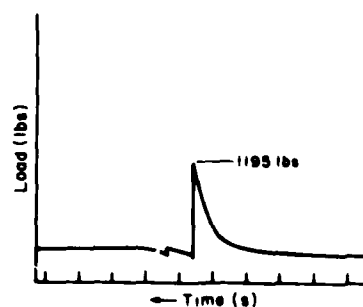
Figure B9. Sample D15 (time interval 1s)
