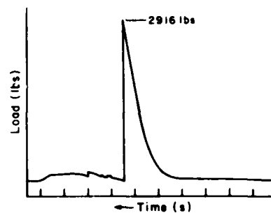
Figure B1. Sample A15 (time interval 1s).
