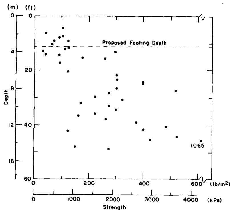
a. Strength vs depth.
