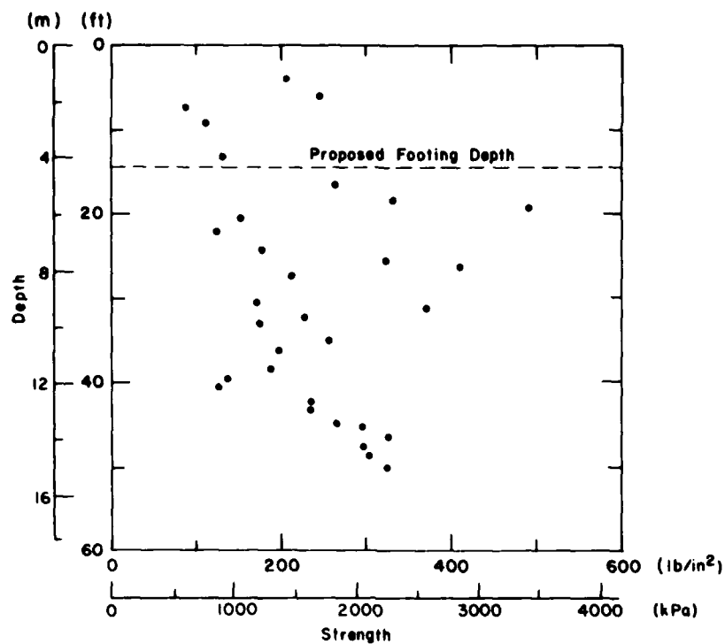
a. Strength vs depth.
