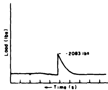
Figure B10 Sample E19 (time interval 1s)
