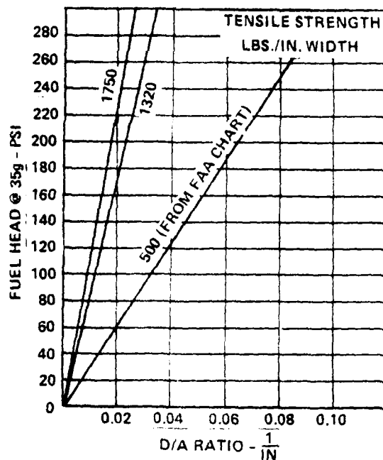
Figure 3-2. Tensile Strength Versus Hydrostatic Head and D/A Ratio
