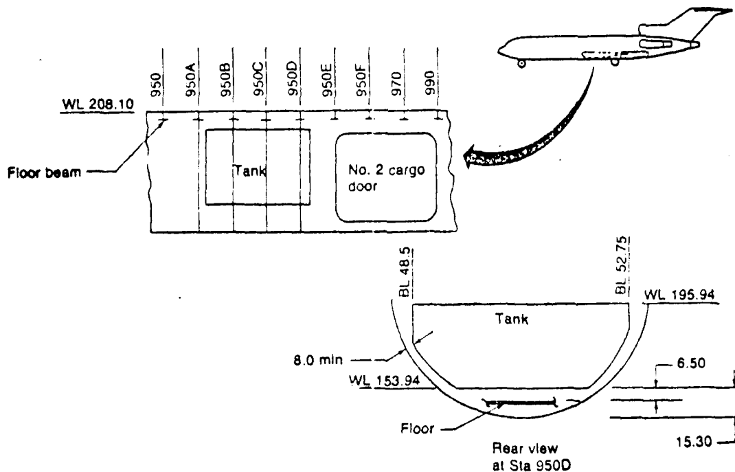
Figure 2-2. Fuel Tank General Arrangement
