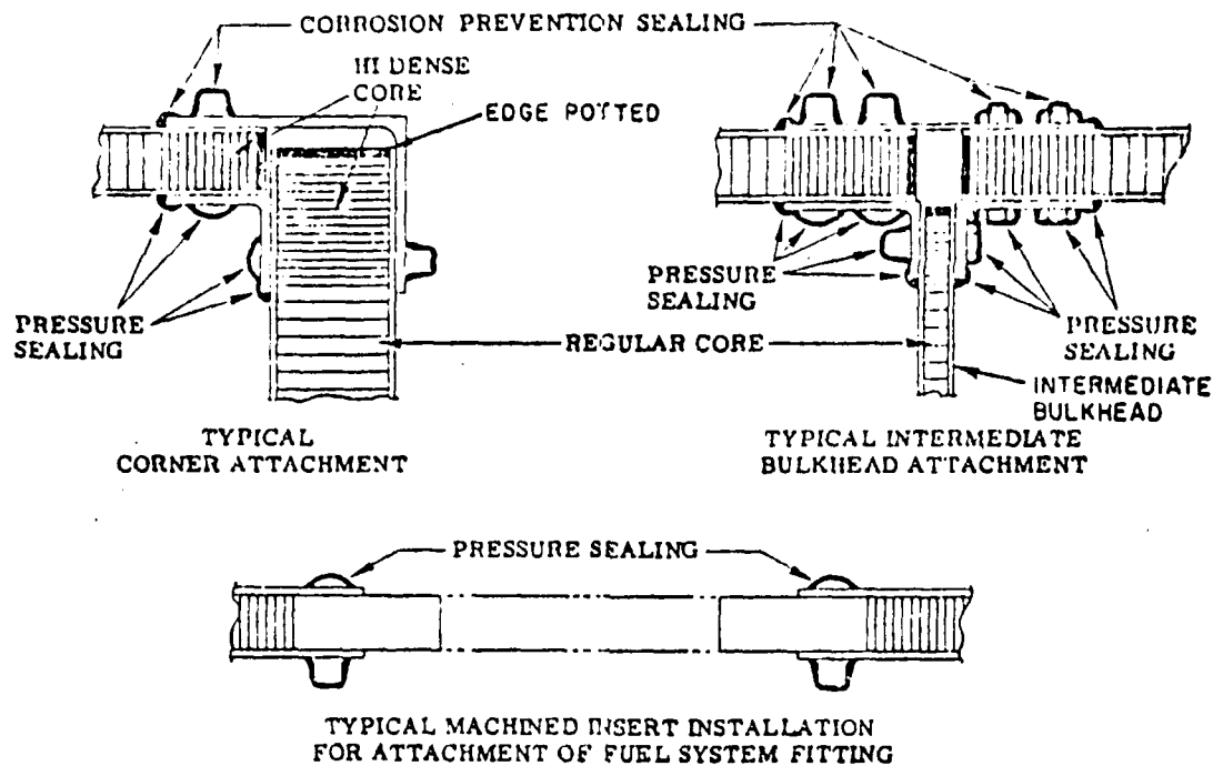
Figure 2-3. Fuel Tank Construction
