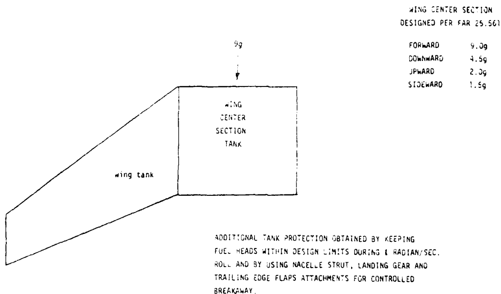
Figure 2-1. Fuel Tank Load Factors
