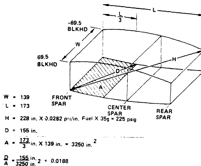
Figure 3-1. Derivation of Cell Design Factors
