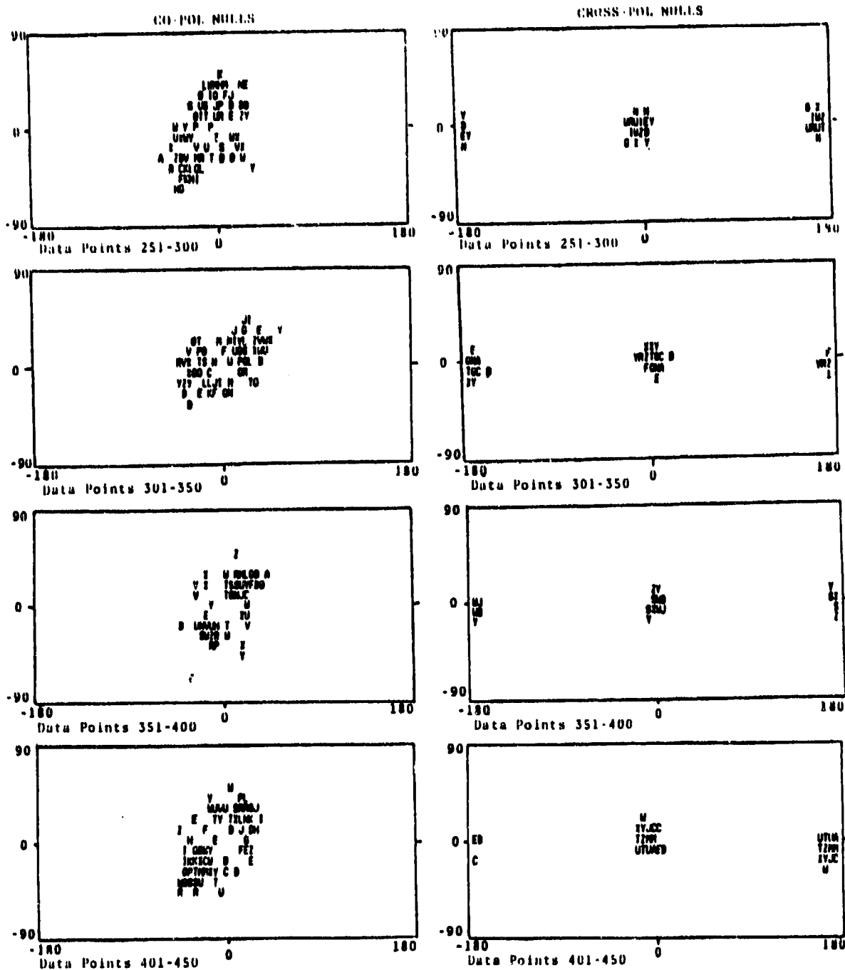
FIGURE 9c - Clutter Polarization Nulls Elevation Angle = 3.3 Data Points 251-450
