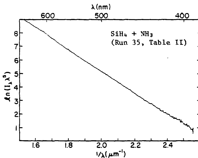
Figure 7. Emission spectra (plotted as \ln(I_\lambda \lambda^5) vs. 1/\lambda ) of reaction flame measured with an optical multichannel analyzer (OMA).
