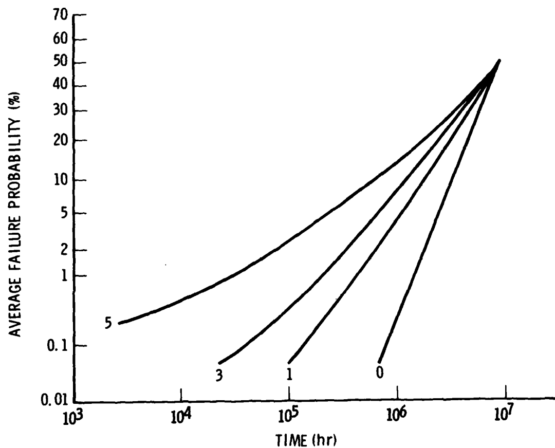
Fig. 2. Estimated Average Failure Probability as Function of Operating Time at 50°C Inferred From Accelerated Aging. The curve designated 0 is the cdf of a lognormal pdf with parameters \tau_M = 10^7 hr and \sigma = 1.00 (see text).
