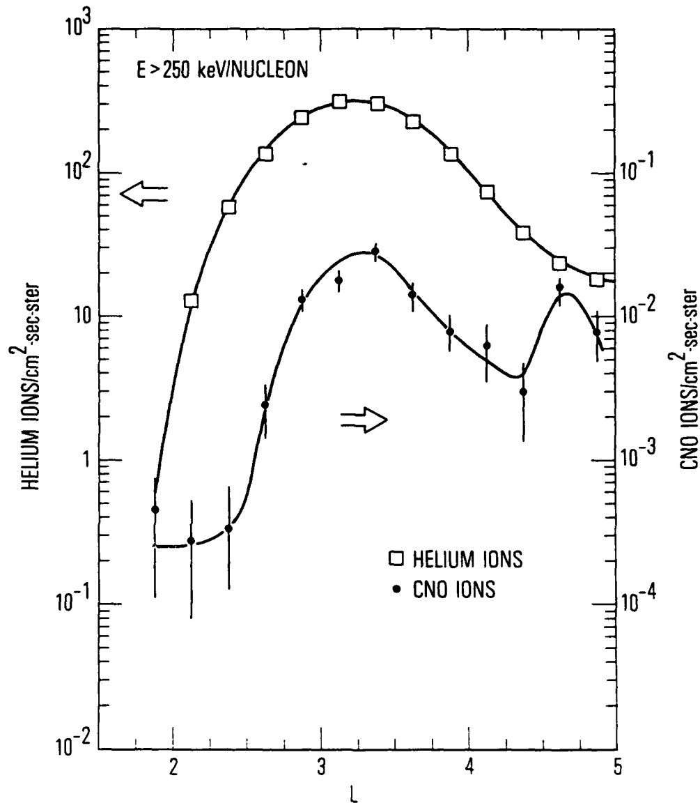
Figure 1. Flux profiles are shown for CNO and He ions as a function of L value for E > 250 keV/nucleon and 0.15 < B < 0.20 gauss. The statistical uncertainty in the He data points is smaller than the symbol; the CNO error bars are shown explicitly. The curves through the points are to guide the eye.
