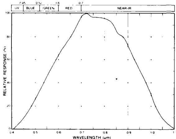
1B-33a. METEOSAT visible channel normalized sensor response curve.
