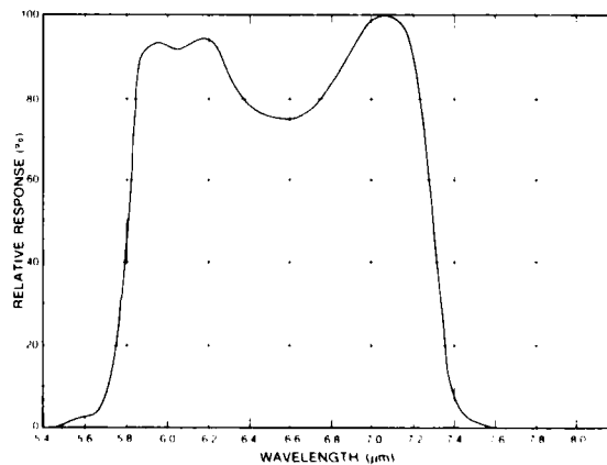
1B-33d. METEOSAT water vapor channel normalized sensor response curve.
