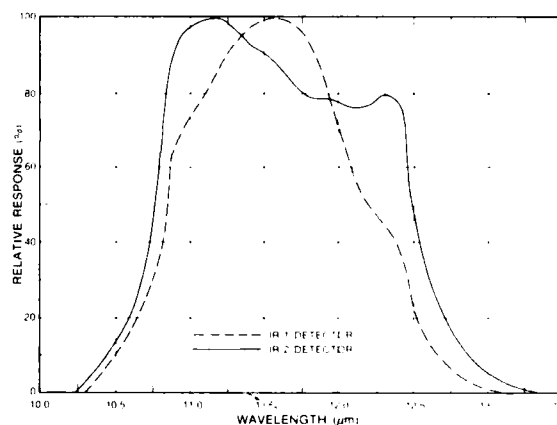
1B-33b. METEOSAT infrared channel normalized sensor response curve.
