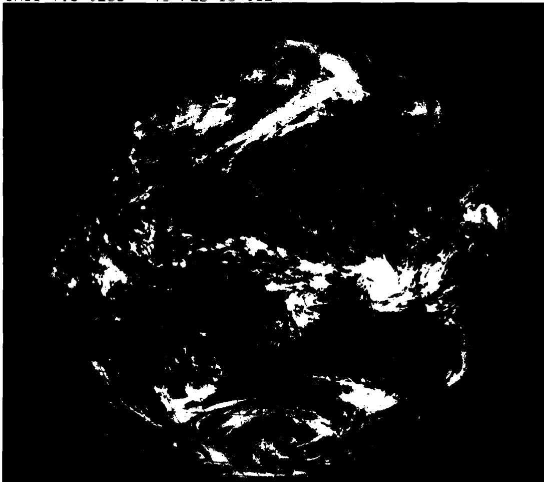
IB-26a. GMS. Visible Picture, 0.7 n mi Resolution, 0300 GMT 15 February 1979. (Photo Courtesy of Japan Weather Association.)
