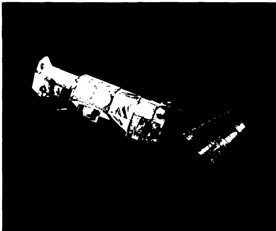
1A-15a. The Block 5D satellite is an integrated spacecraft in that the launch vehicle upper stage remains attached to and provides support for the satellite in orbit. The satellite itself is a five-sided box-like structure (the prototype for TIROS-N) in which four of the five sides are equal in size and contain thermal control louvers, while the fifth side is wider and contains the Earth-viewing sensors. A large solar power panel is attached to one end of the spacecraft; it rotates once each orbit so that it is always oriented toward the sun during the daylight portions of the orbit.
