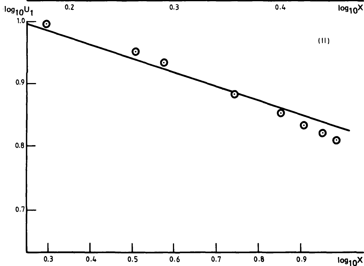
FIG. 10 FREE STREAM VELOCITY VARIATIONS OF EQUILIBRIUM LAYERS. I. Ludwig & Tillmann (1949) mild adverse pressure gradient flow. II. Clauser (1954) Flow 1.
