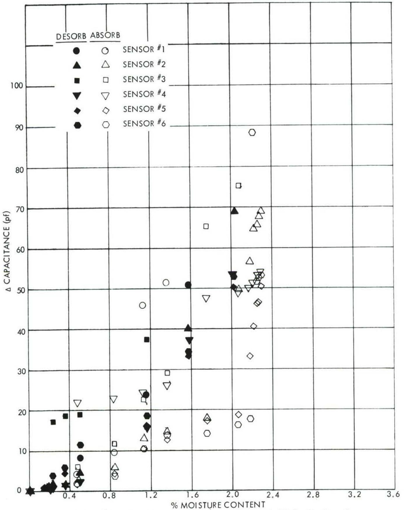
Figure 58. Δ Capacitance Versus Moisture Content for 13-Ply Specimen C
