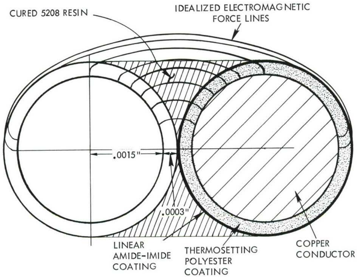
Figure 1. Capacitance Sensor Detail
