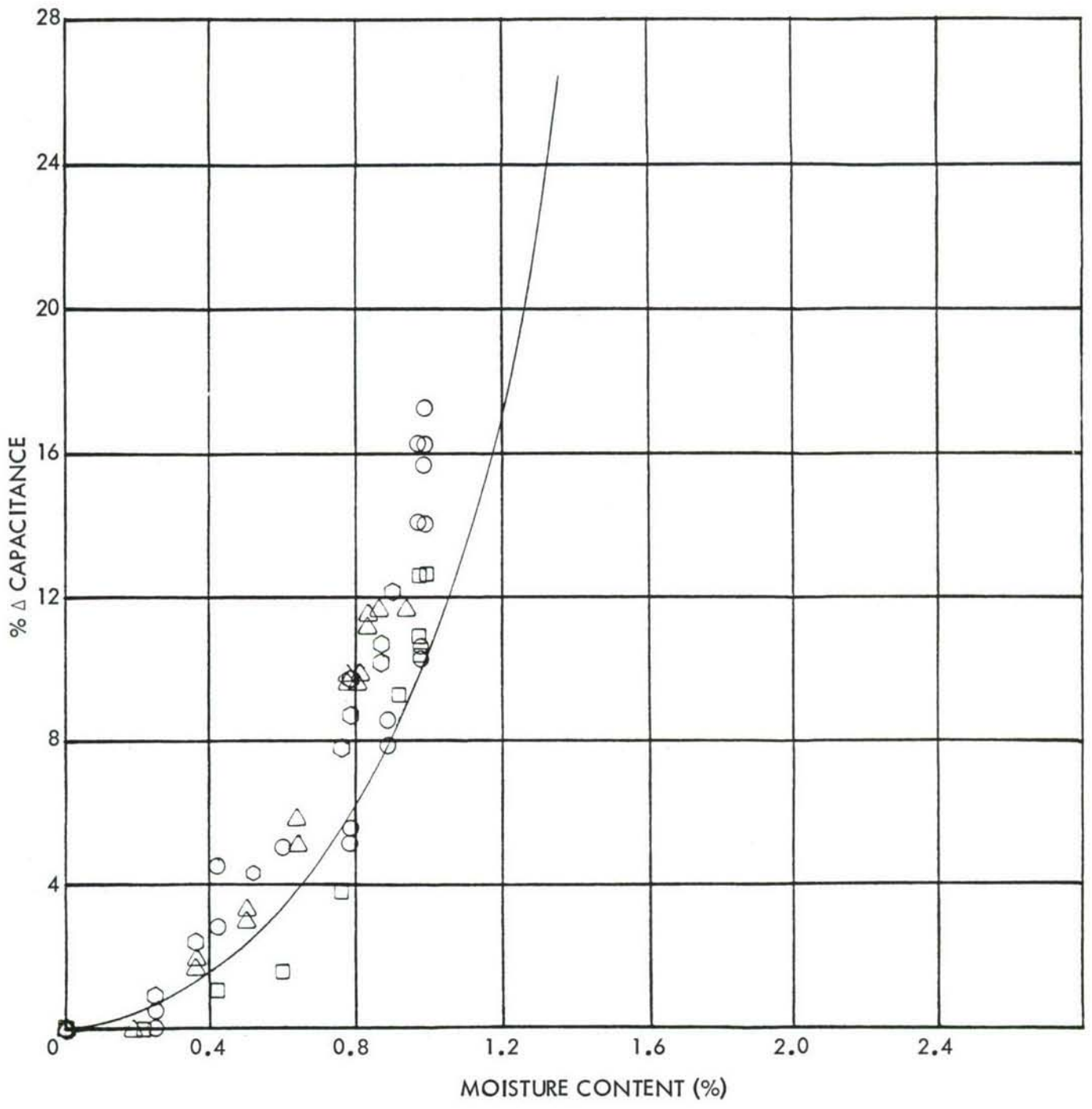
Figure 48. Moisture Content/Capacitance Correlation for Specimen DFD
