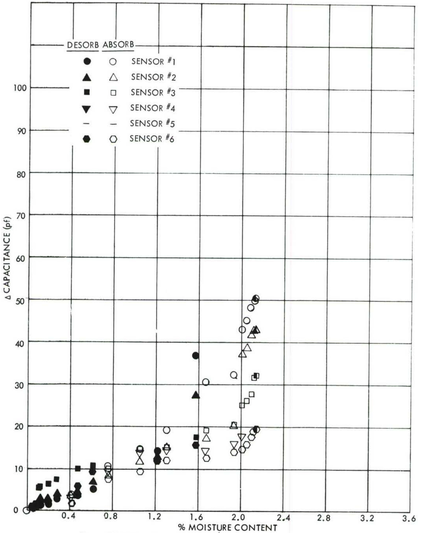
Figure 57. \Delta Capacitance Versus Moisture Content for 13-Ply Specimen B
