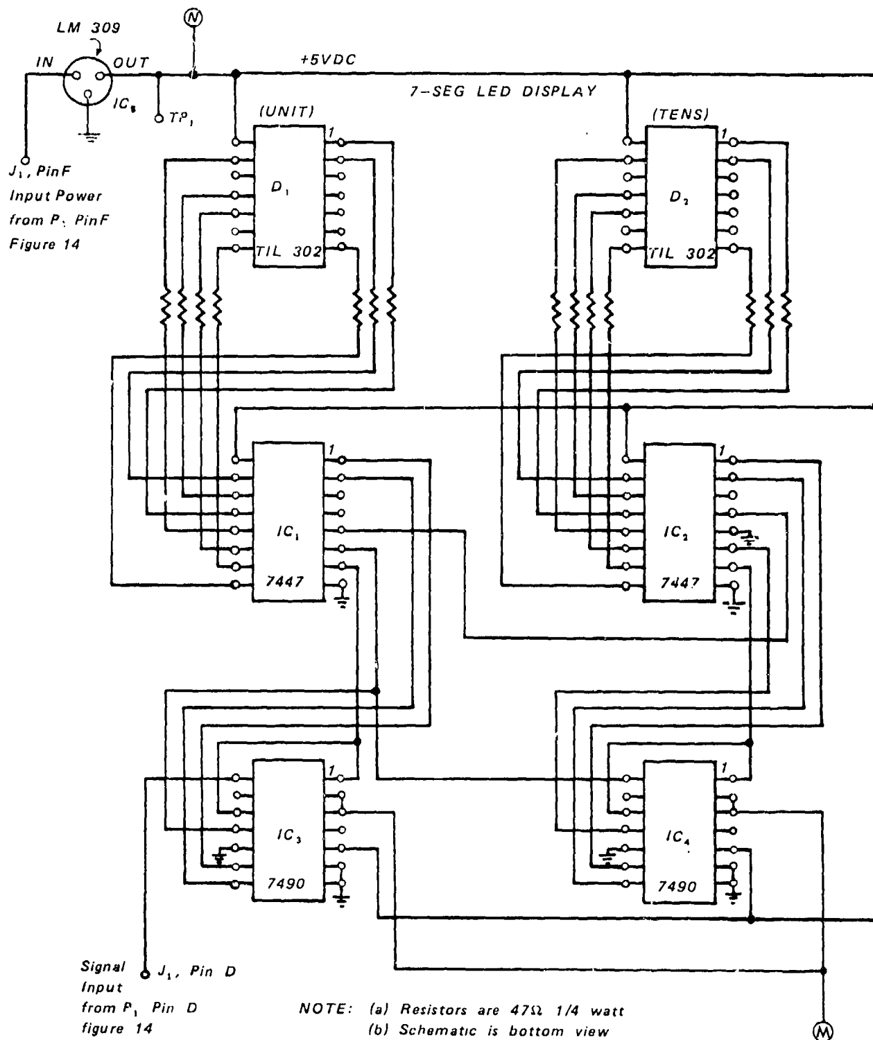
Figure 16. Digital Electronic System Schematic.
