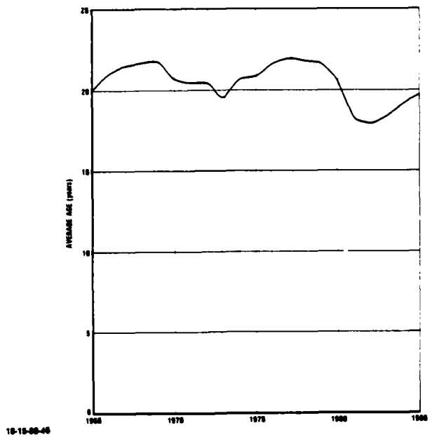
FIGURE 27. Auxiliary Support Vessels—Average Age
