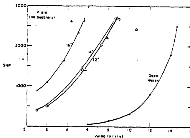
Figure 7. Shaft horsepower vs velocity for plate ice with no bubblers in operation. 1 to 5 in. of snow cover, n = 1.2 to 1.5 (0.05 to 0.11)
