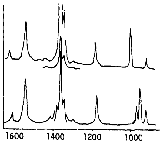
Figure II-5. Raman Spectra of Solid 1,3,5-Trinitrobenzene and 1,3,5-Trinitrobenzene-d 3 in the Region 100-800 cm -1 , excited by the 4880Å line of an Argon Ion Laser (Shurvell et al. , 1969) Reproduced by permission of the National Research Council of Canada
