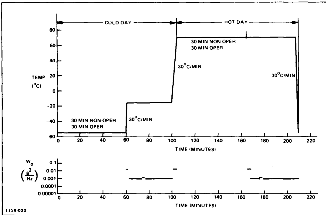
Figure 19 "B" V/STOL Deck Launched Intercept Environmental Profile
