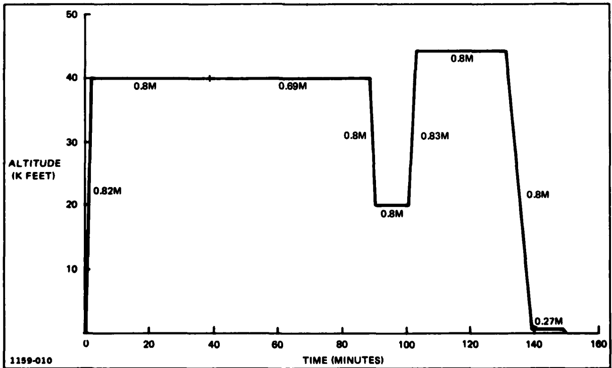
Figure 10 "B" V/STOL Subsonic Surface Surveillance Mission Profile
