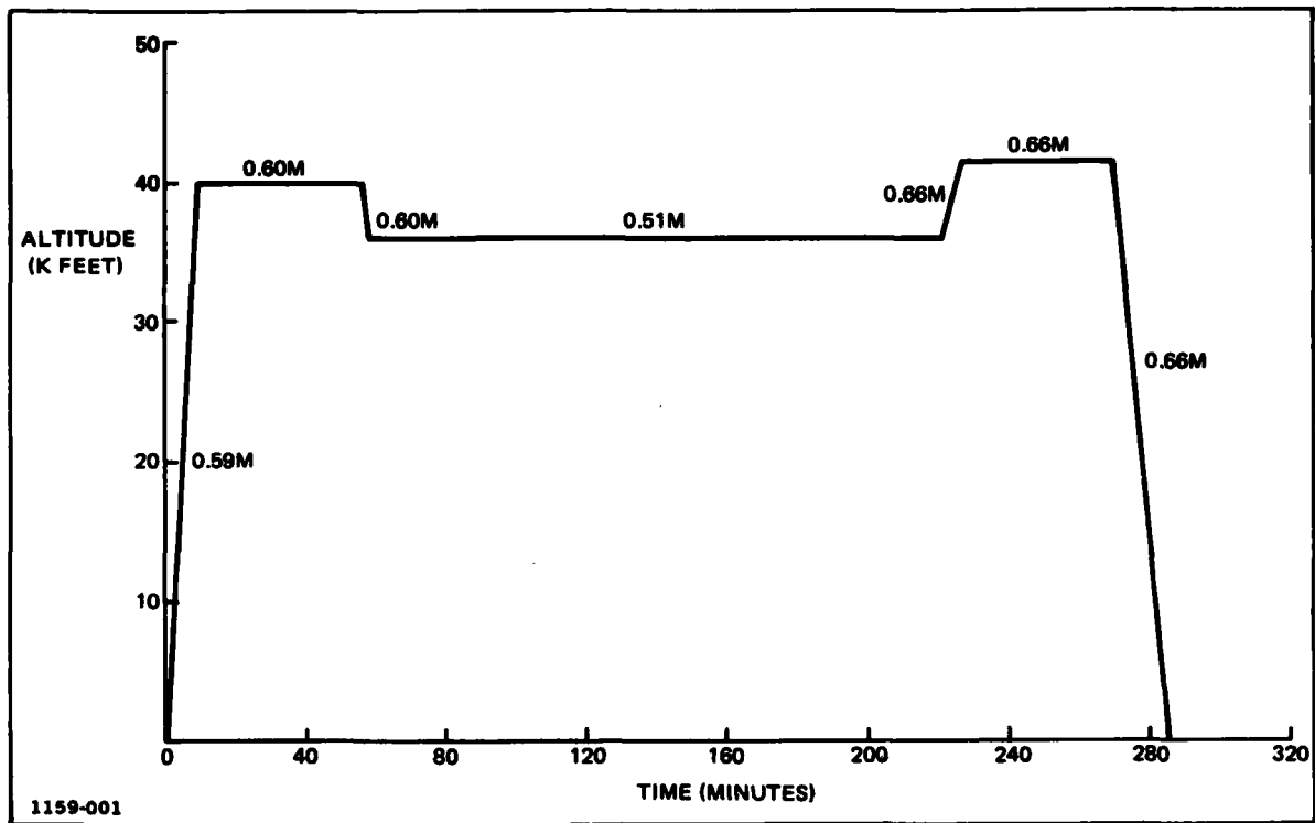
Figure 1 "A" V/STOL Airborne Early Warning Mission Profile
