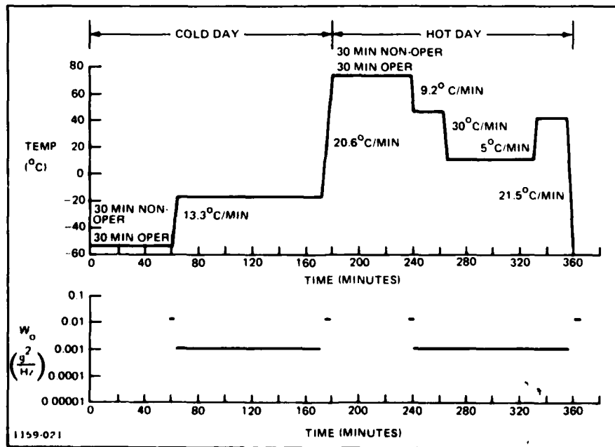
Figure 20 "B" V/STOL Subsonic Surface Surveillance Environmental Profile
