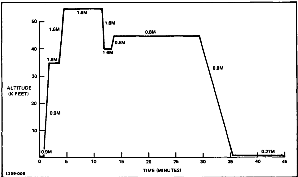
Figure 9 "B" V/STOL Deck Launched Intercept Mission Profile
