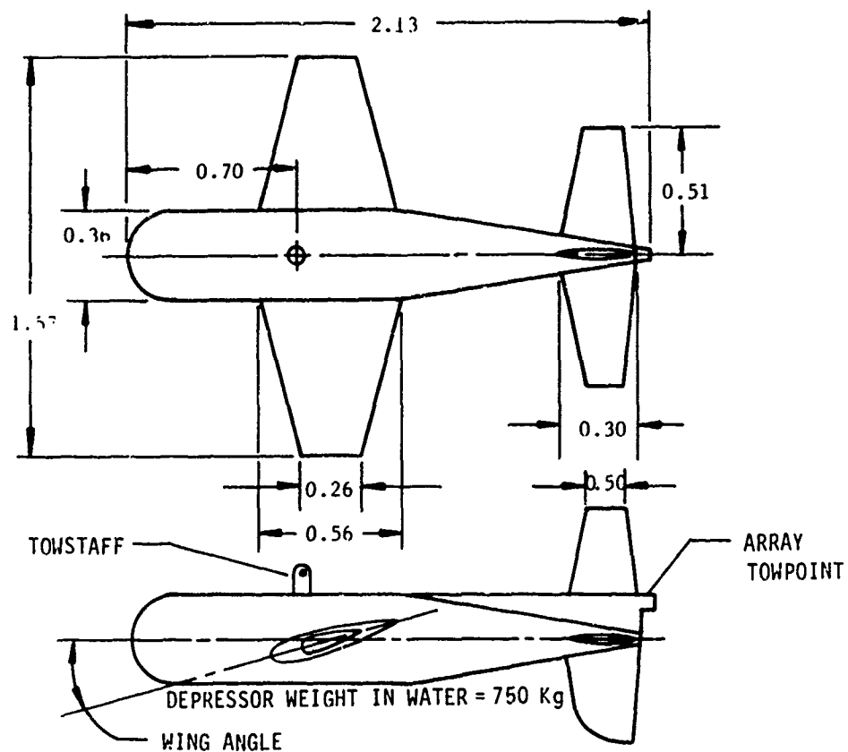
Figure 2 - DTNSRDC Depressor
