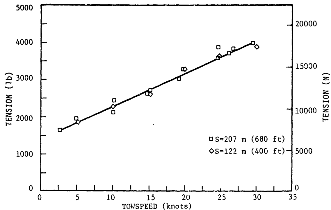
Figure 10a - Tension
