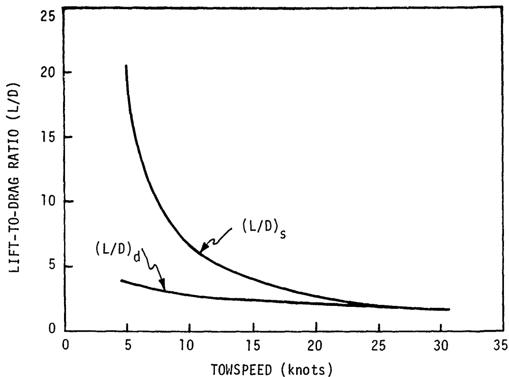
Figure 13 - Lift-to-Drag Ratios for Various Towspeeds
