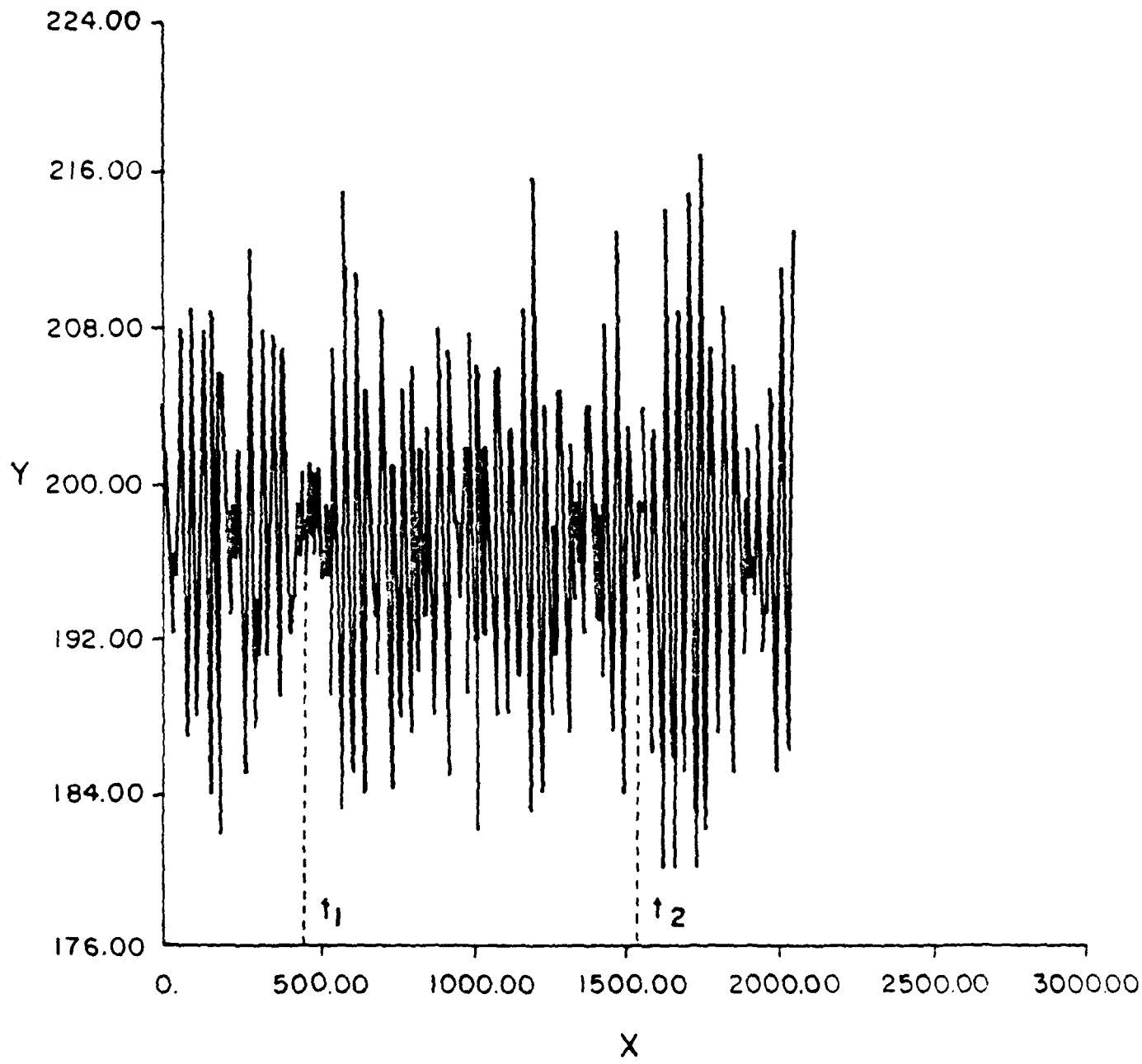
Fig. 3. A typical flow (high) calibration file with t_1 and t_2 shown for illustration only. Flow (Nicolet units) is plotted on the vertical axis and time (Nicolet units) for a flow of 1 l/s; each time unit represents 10 ms. Note that the signal noise is exaggerated by the zero-suppression and expanded scale of the vertical axis.
