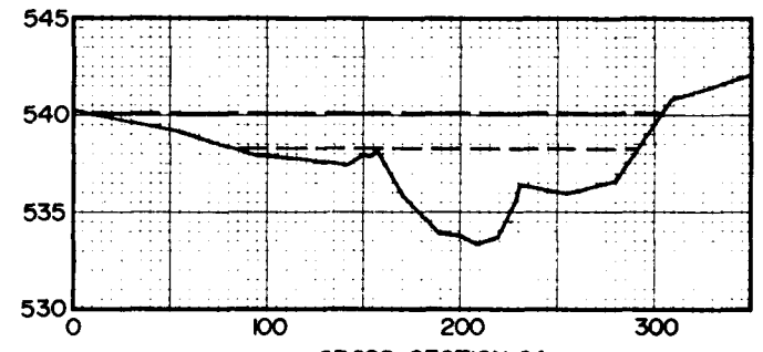
CROSS SECTION 29 MILE 21.46
