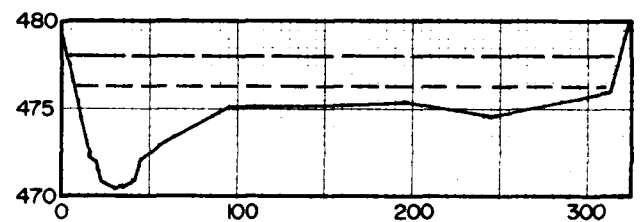
CROSS SECTION 24 MILE 16.50
