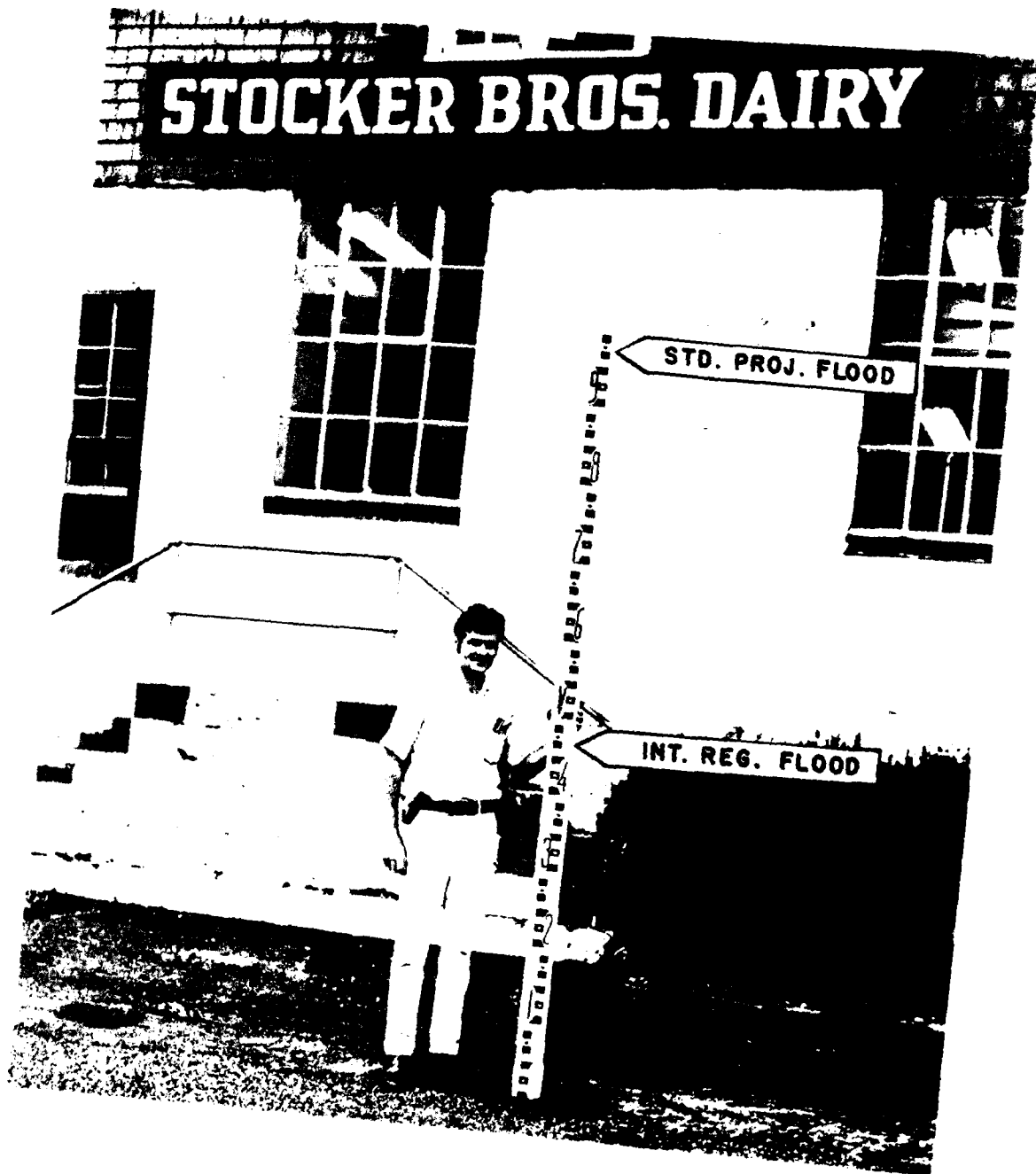
FIGURE 9 - Future flood heights at the Stocker Bros. Dairy in Zucksville, Pa.
