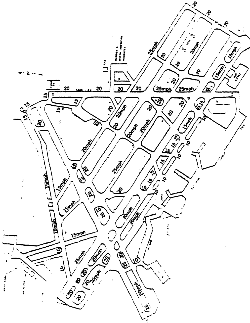
Exhibit 4C Lambert-St. Louis International Airport GENERALIZED TAXIWAY SPEEDS FOR ARRIVALS AND DEPARTURES ON RUNWAY 24 Peat, Marwick, Mitchell & Co. June 1980
