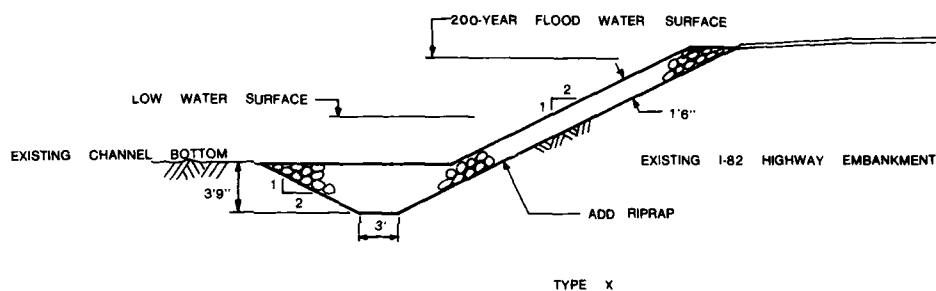
TYPICAL SECTION FOR I-82 HIGHWAY BANK PROTECTION IMPROVEMENT
