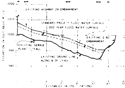
RIGHT BANK LEVEE (BELOW MOXEE BRIDGE) PROFILE
