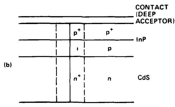
Figure 8. Hypothetical electrical properties at the InP/CdS thin film grain boundaries (a) after InP deposition and (b) after InP deposition and subsequent contact anneal of deep acceptors.
