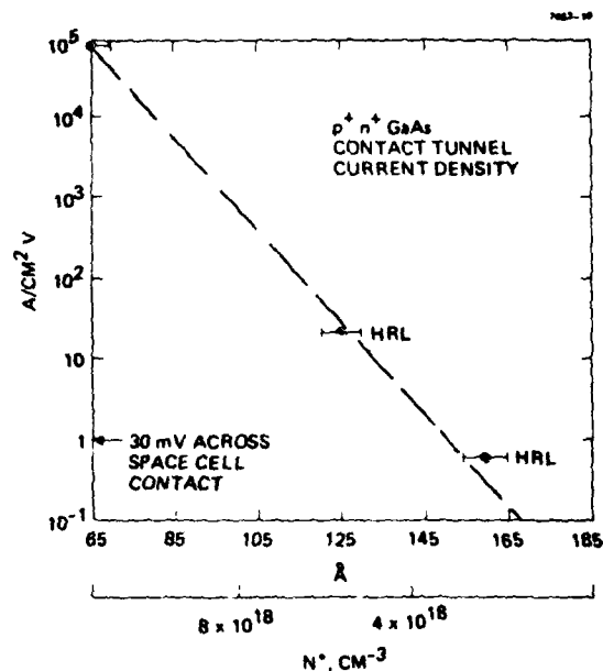
Figure 3. Gallium arsenide tunnel junction current density per volt as a function of barrier width.
