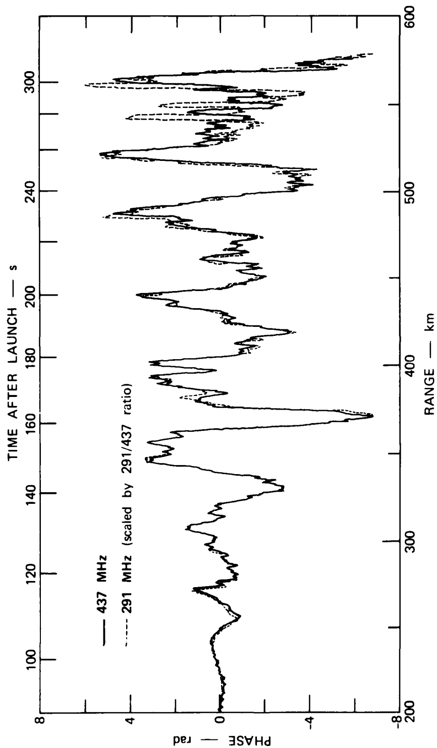
FIGURE 4 PHASE DATA
