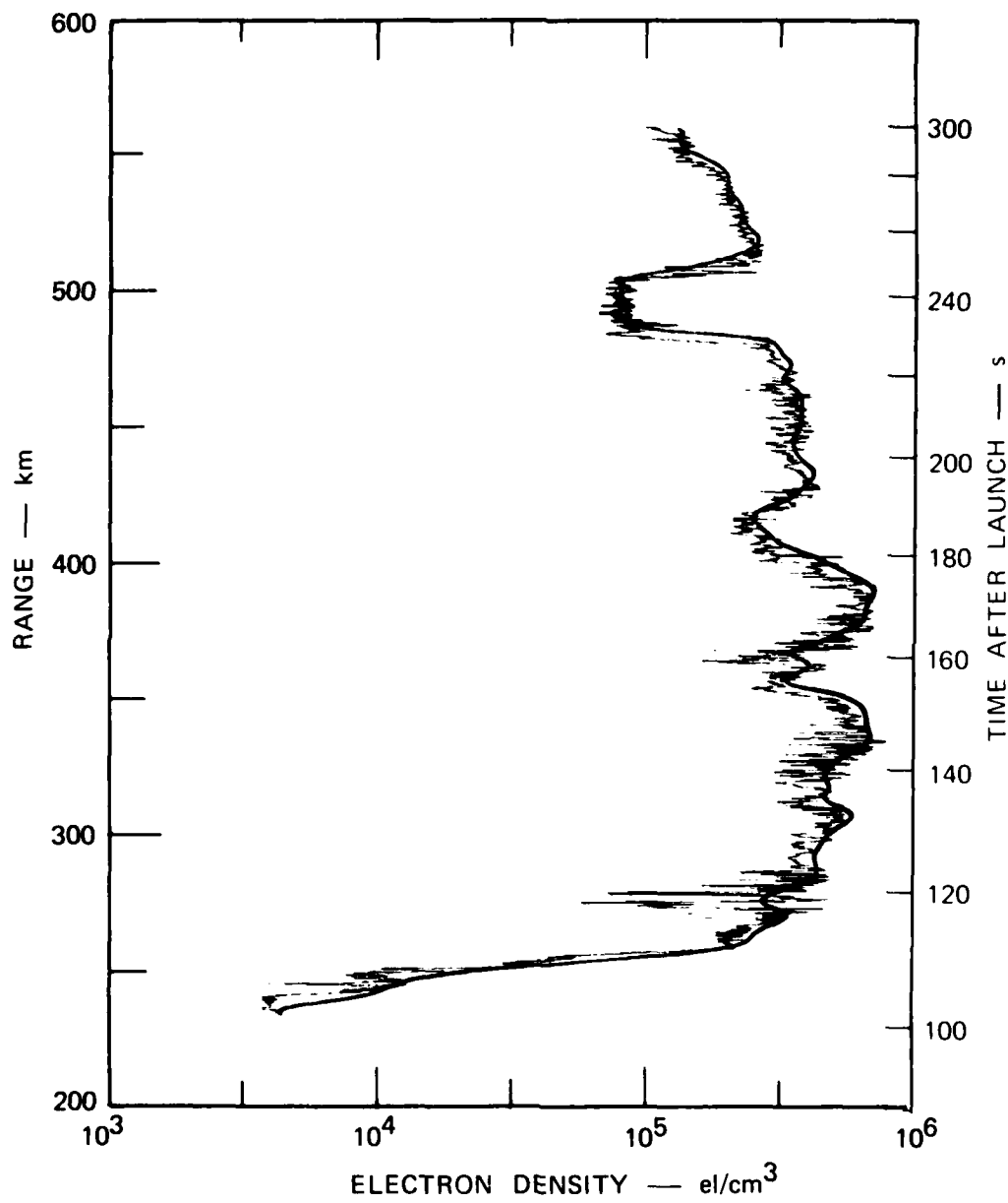
FIGURE 11 UPLEG ELECTRON-DENSITY PROFILE DERIVED FROM THE LANGMUIR PROBE DATA
