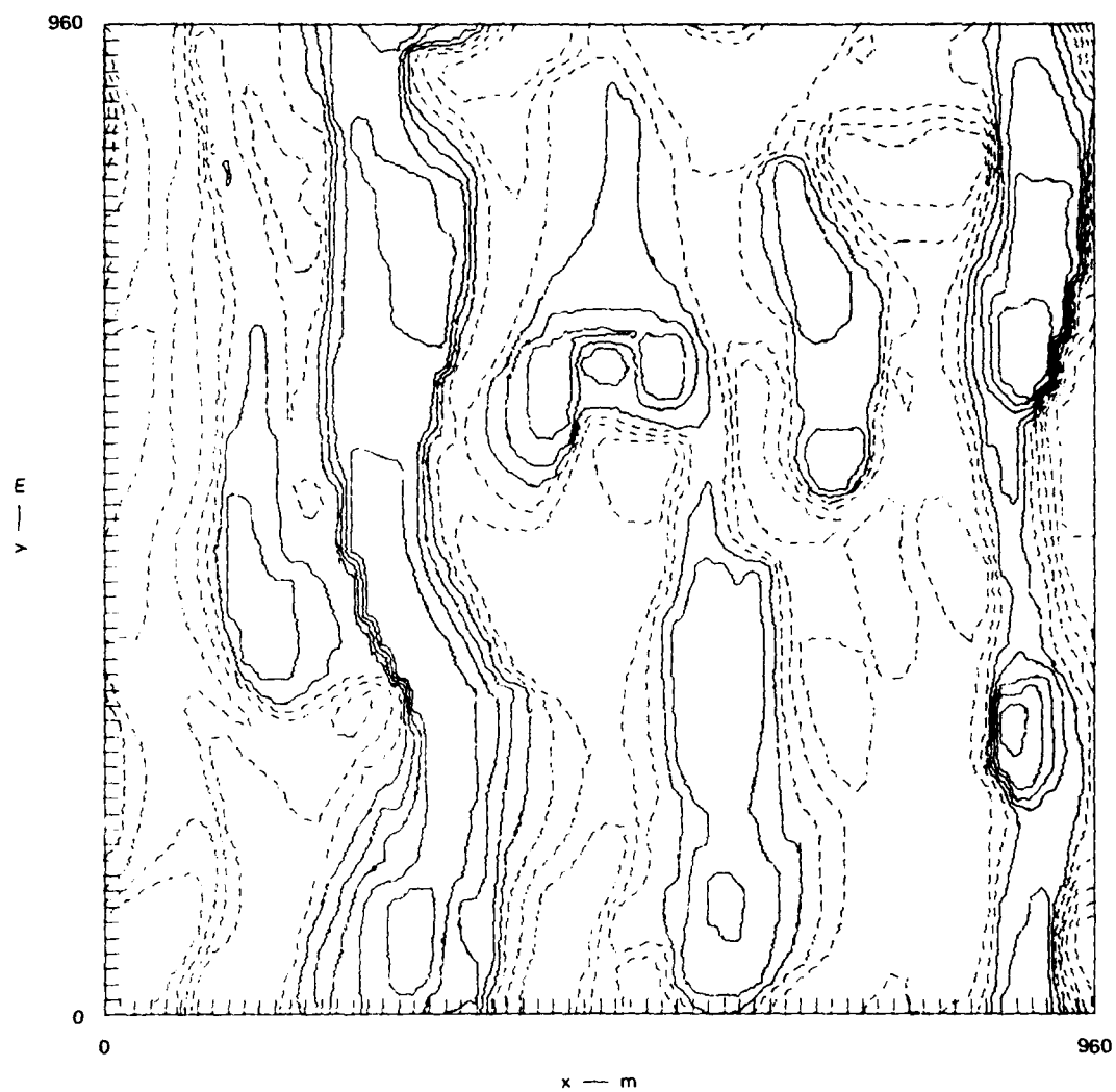
FIGURE 2 DENSITY CONTOURS AT t = 2000 s
