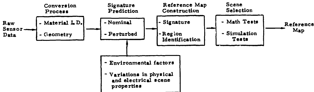
Figure 4. Reference map construction and scene selection process
