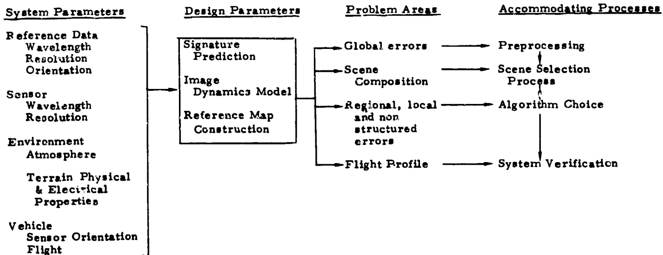
Figure 2. Overall map-matching system design
