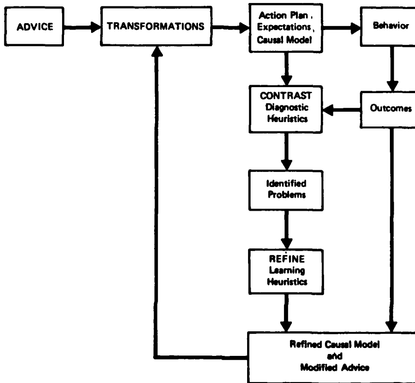
Figure 5--Knowledge-refinement strategy
