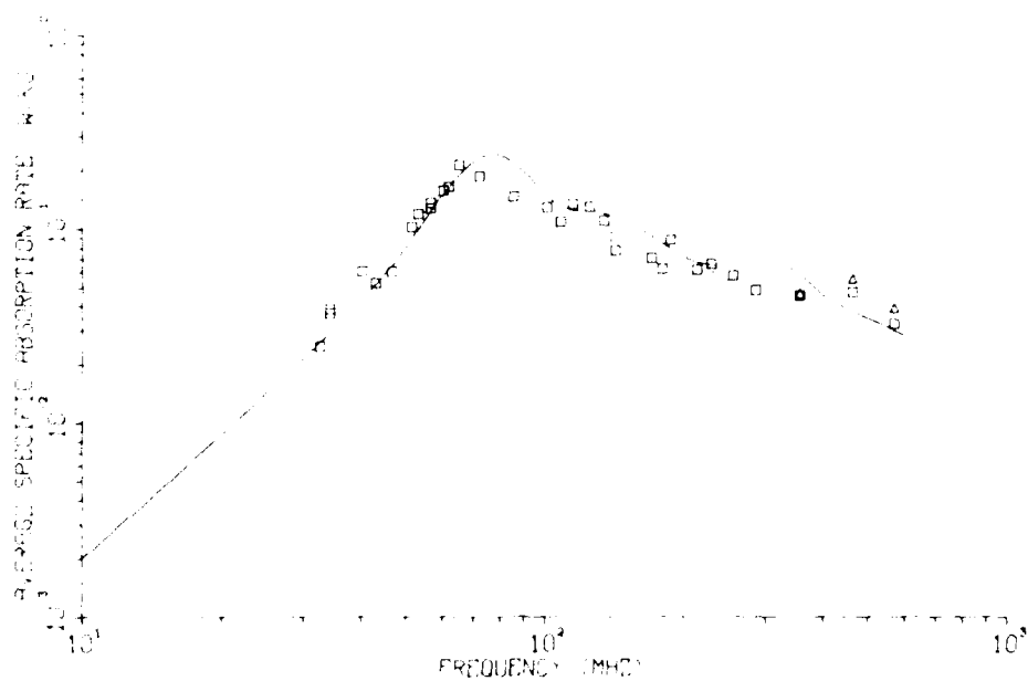
Fig. 3. Whole-body SAR for homogeneous model of man in free space \vec{E} \perp \vec{I} \perp \vec{k} front-to-back, incident intensity = 1 \text{ mW/cm}^2 . Squares represent experimental points for saline-filled figurines. Triangles represent experimental values for figurines containing biological phantom mixtures.
