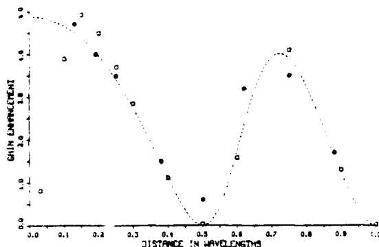
Fig. 9. Variation of gain enhancement with spacing for a half-wave dipole in front of a flat reflector. Squares represent numerical solutions for enhancement of SARs in man at 77 MHz ( L/\lambda = 0.45 ). Solid circles represent experimental values for anatomically scaled figurines at L/\lambda = 0.417 .
