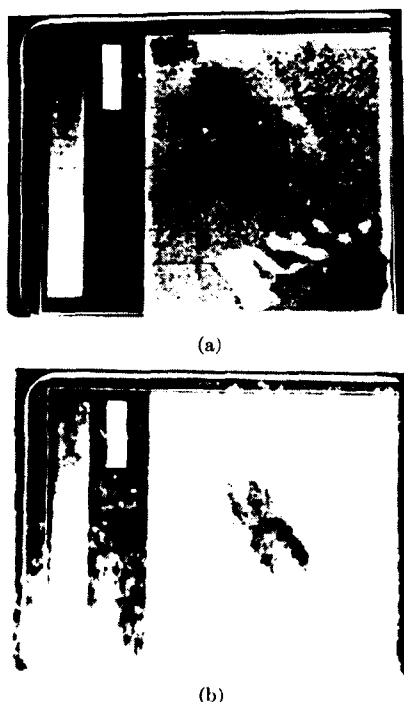
Fig. 10. Thermographic recording of the central section of an 18.4-cm biological-phantom figurine; free-space irradiation of 710 MHz (temperature of the body before irradiation \sim 7 \frac{1}{2}^{\circ}\text{C} ). (a) After irradiation in the \mathbf{E} \parallel \hat{\mathbf{L}} configuration for 10 min at 100 mW/cm 2 ; baseline 8^{\circ}\text{C} ; 3^{\circ}\text{C} full scale. (b) After irradiation in the \mathbf{H} \parallel \hat{\mathbf{L}} configuration for 10 min at 100 mW/cm 2 ; baseline 8^{\circ}\text{C} ; 3^{\circ}\text{C} full scale.
