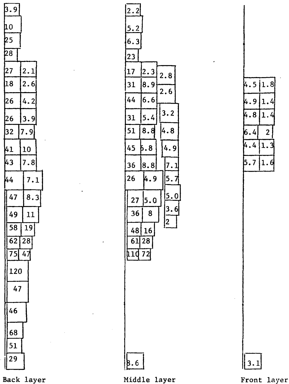
Figure 4. Local SAR values (watts/kg per \text{mW/cm}^2 ) \times 100 for inhomogeneous model of man with vertical polarization at 80 MHz.
