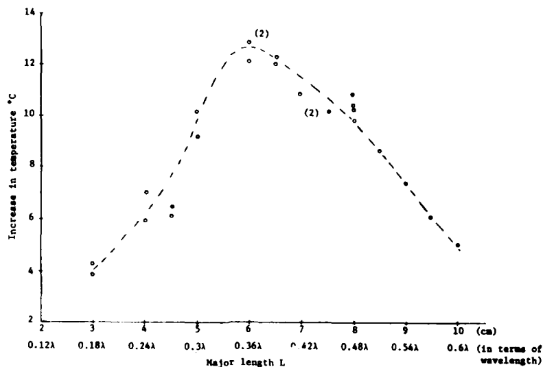
Fig. 2. Temperature rise in saline-filled prolate spheroids with an aspect ratio L/2b of 6. Frequency, 710 MHz; irradiation time, 5 min; incident power density, 100 mW/cm 2 ; polarization, E \parallel \hat{L} .
