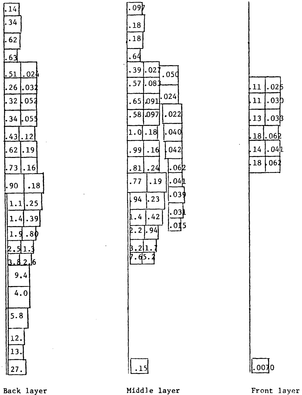
Figure 6. Local SAR values (watts/kg per \text{mW}/\text{cm}^2 \times 100 ) for inhomogeneous model of man standing on a ground plane at 10 MHz.
