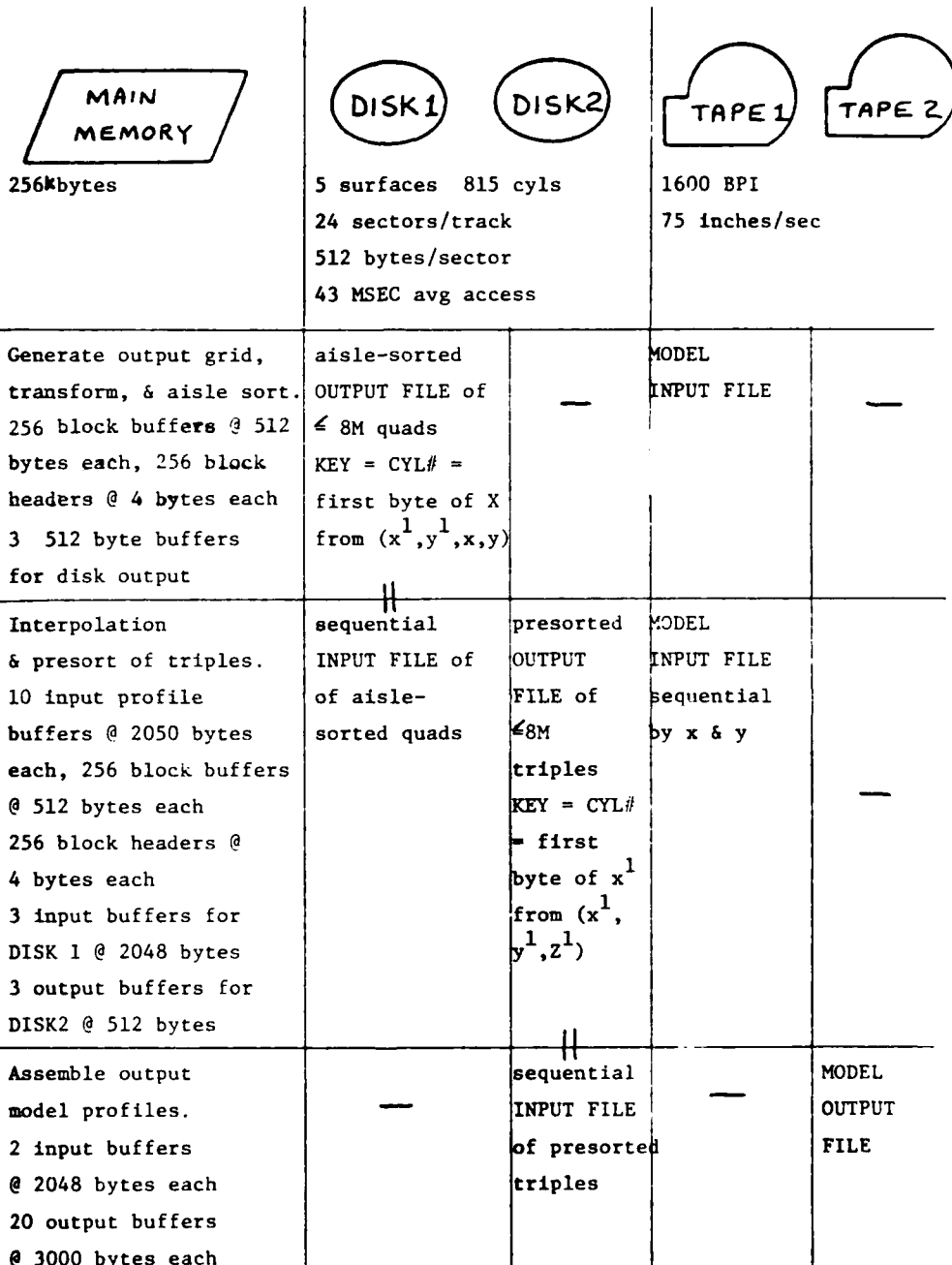
Figure f. Peripheral flow diagram for the refined MiniMARS algorithm
