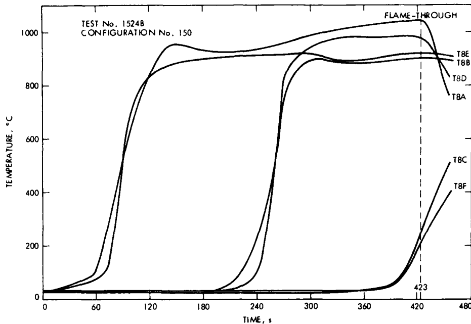
Figure 9-16. Spiral-Wound, Crimped Stainless-Steel Ribbon Arrestor Ethylene/Air Mixture Sustained Burning First Test Results
