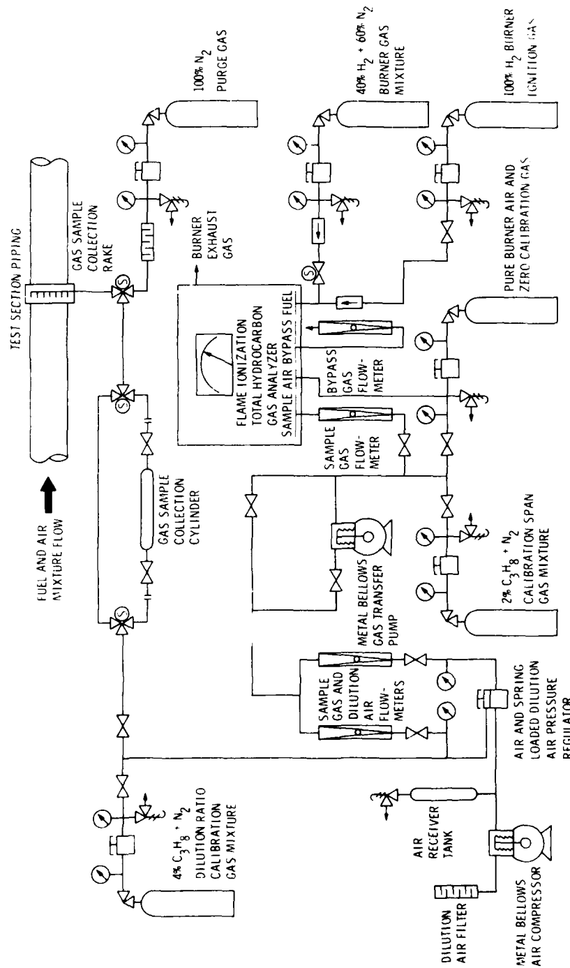
Figure 4-9. Hydrocarbon Gas Sample Analyzer and Air Filtration System Schematic Diagram
