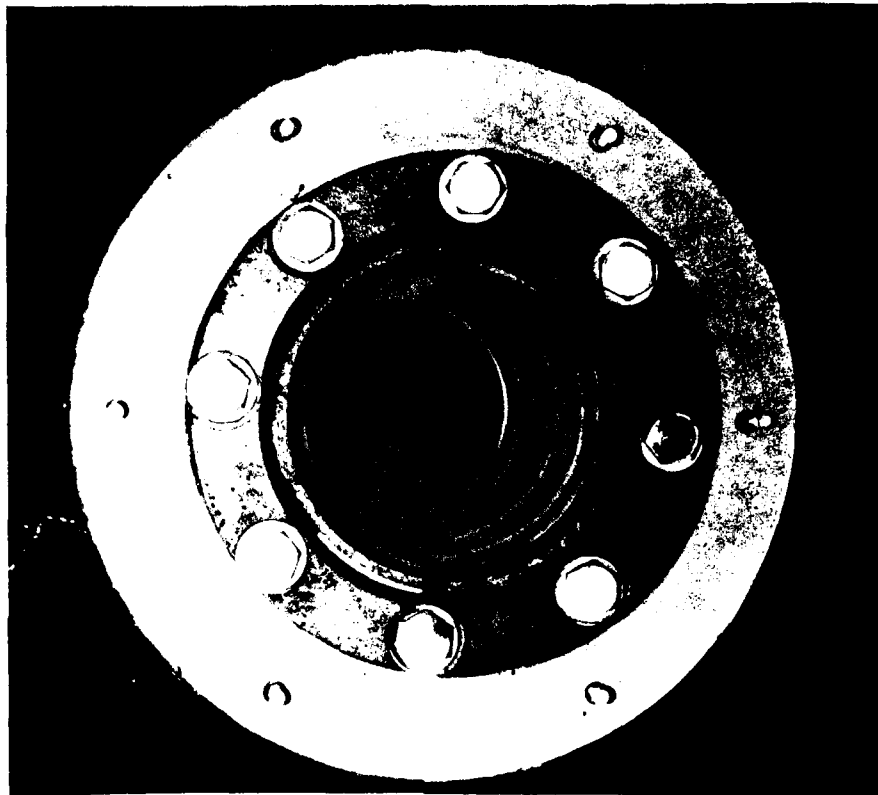
Figure 1. View of the end of the pipe after the test.
