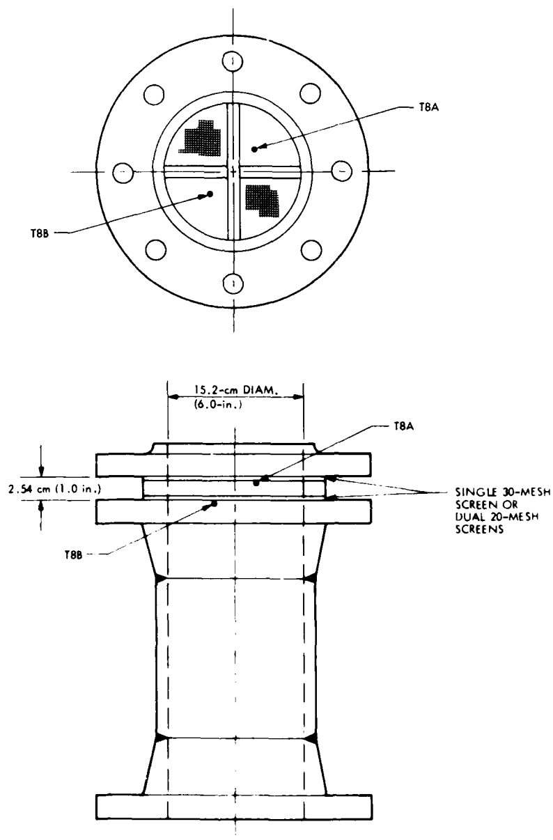
Figure 9-1. Screen-Type Arrestor Test Assembly, 15.2-cm Diameter, Schematic Drawing
