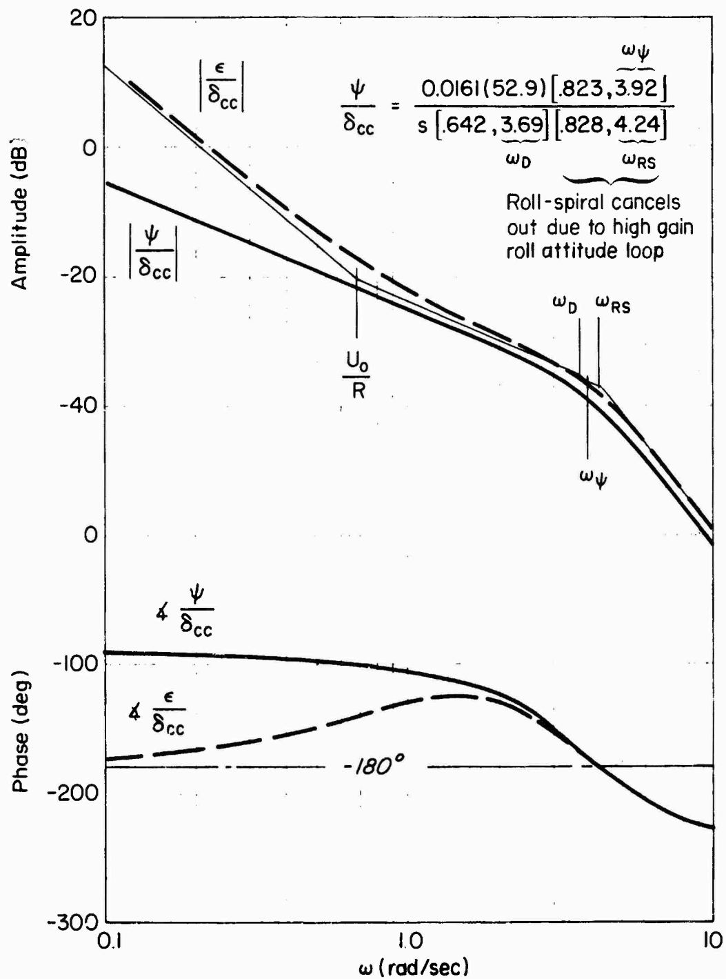
Figure 21. Comparison of Heading Dynamics and Piper Error Dynamics for Wings-Level Turn
