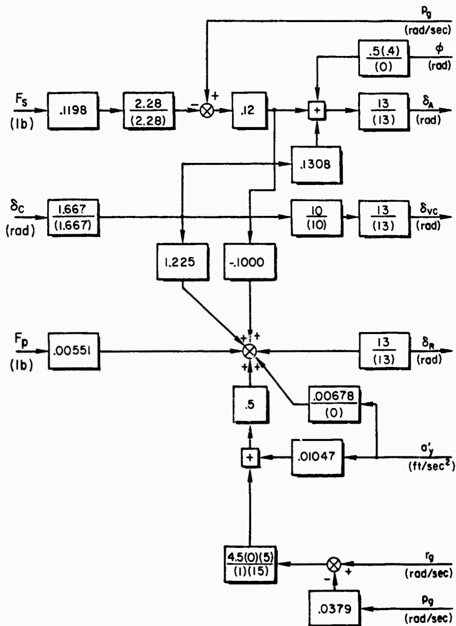
Figure 42. Lateral-Directional Flight Control System, Yaw Pointing ( \beta_1 ) Mode
