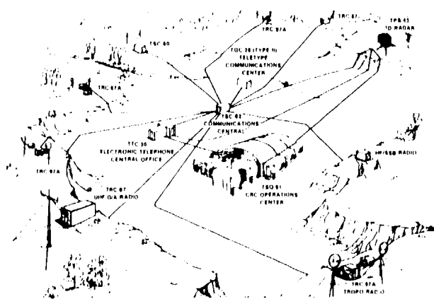
Fig. 10. Cosite Interference
