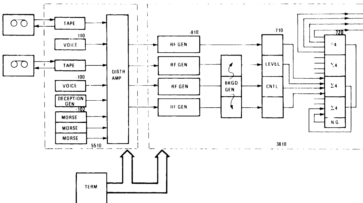
Figure 9. Comms Simulator
