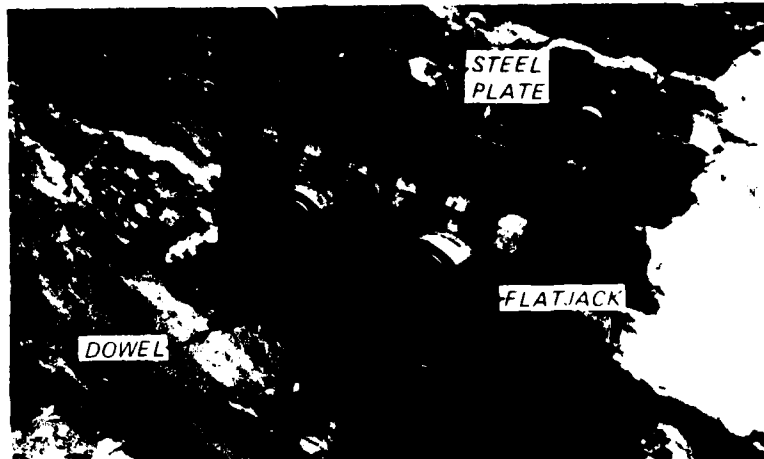
Figure 24. Modified testing apparatus, lock wall pullout tests (Note: plate reversed for photo)
