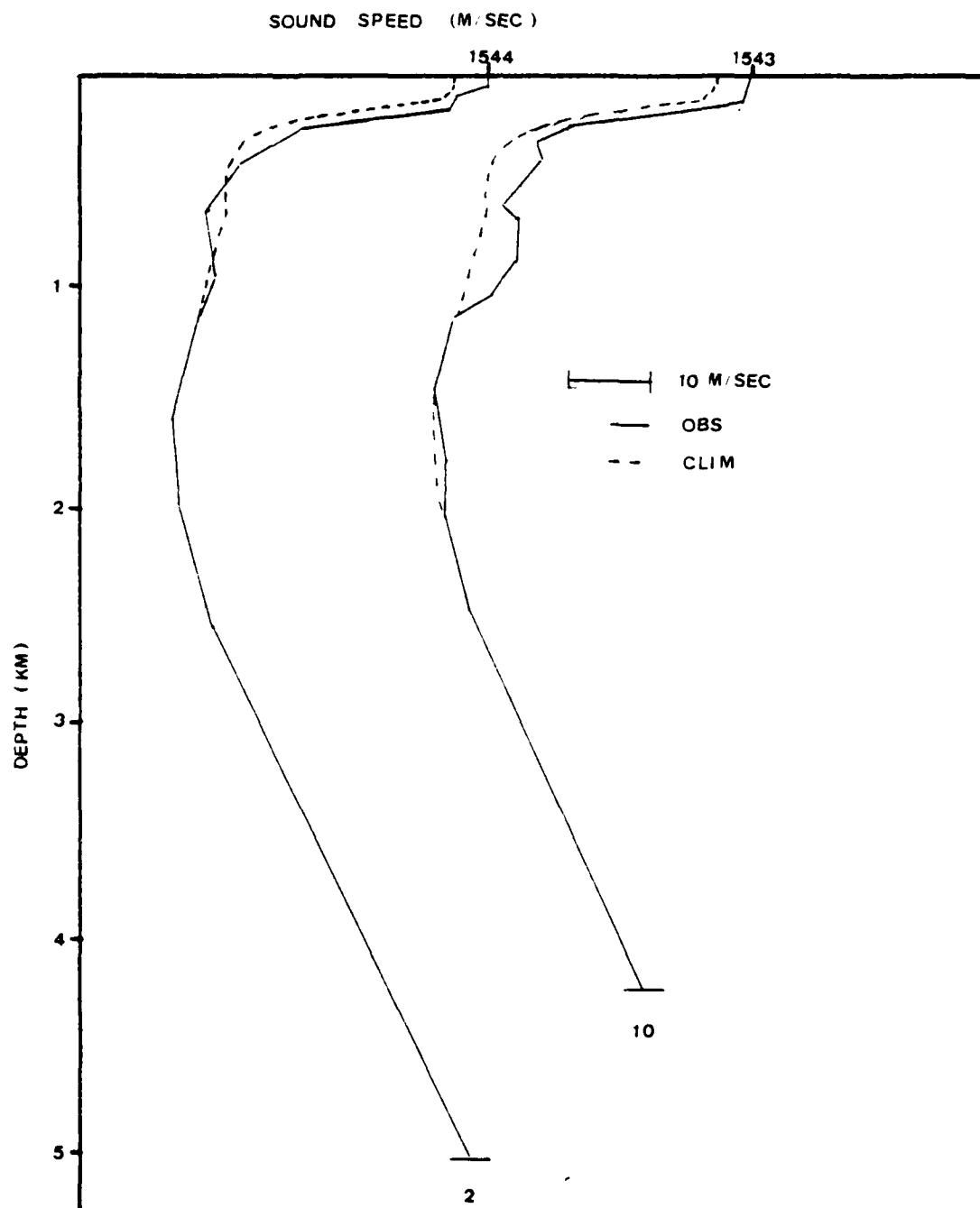
Figure 33. Sound speed profile at Stations 2 and 10, March 1977.
