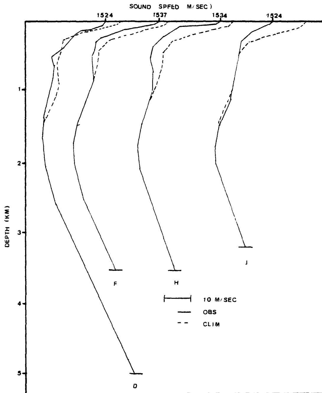
Figure 28. Sound speed profiles in upwelling areas, August 1976.
