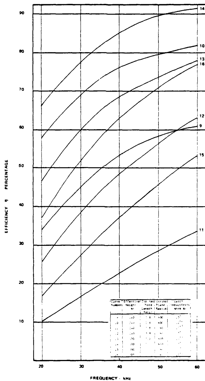
Figure 21. 600 m Tower Systems - Radiation Efficiency
