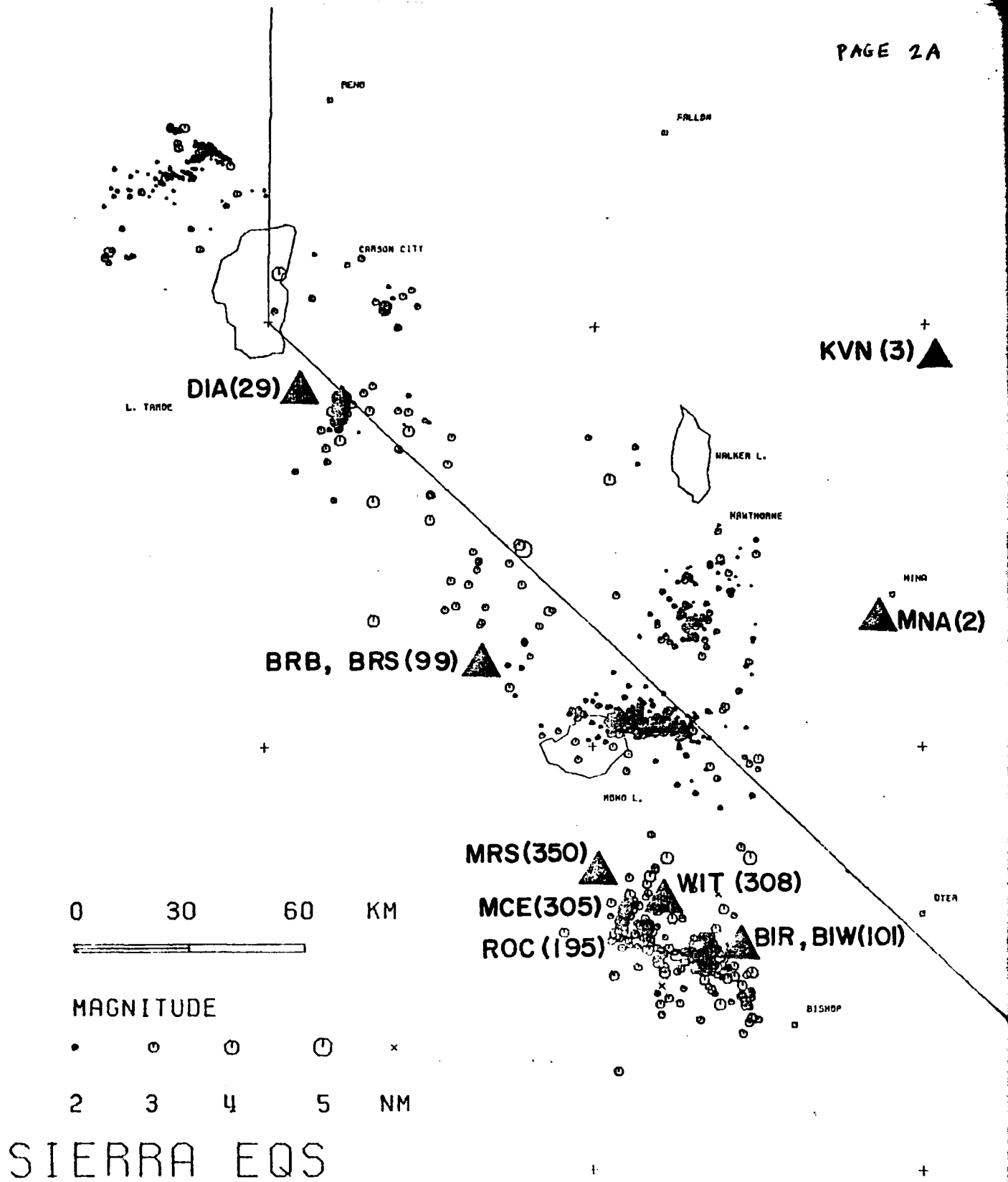
Figure 1.1. Indicating station names where digital data was collected and the number of three-component records obtained at each site. Seismicity 1975-1979 is shown also.
