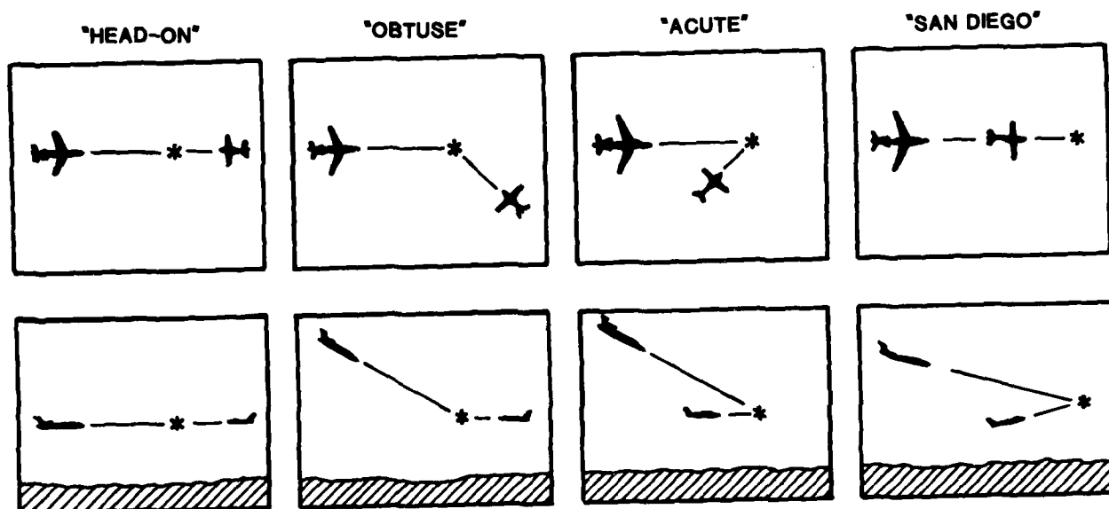
Flight Paths for Lincoln Laboratory Testing of BCAS Surveillance
