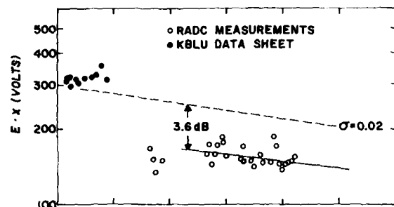
Figure 3. Southern Pacific RR (90° - 100°) Sector Path Profile (lower portion) and Signal Strength-Distance Product
