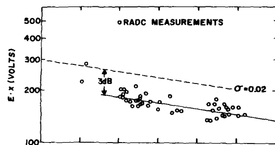
Figure 4. Mohawk Valley (100° - 107.5°) Sector Path Profile (lower portion) and Signal Strength-Distance Product
