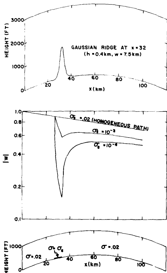
Figure 11. The Attenuation Function |W| on the Surface of the Inhomogeneous Path Shown at the Bottom of the Figure, for Three Values of \sigma_s
