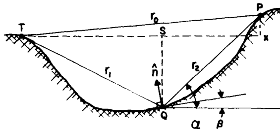
Figure 9. Geometry for the Integral Equation. s and x are the horizontal distances of the scattering point Q and the observer P , respectively, from the source T . \alpha is the slope of r_2 , \beta is the terrain slope at Q , and \hat{n} is a unit vector at Q normal to the terrain
