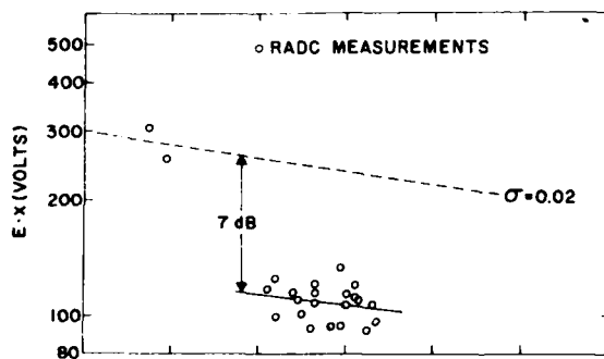
Figure 6. Coyote Peak (110° - 116°) Sector Path Profile (lower portion) and Signal Strength-Distance Product
