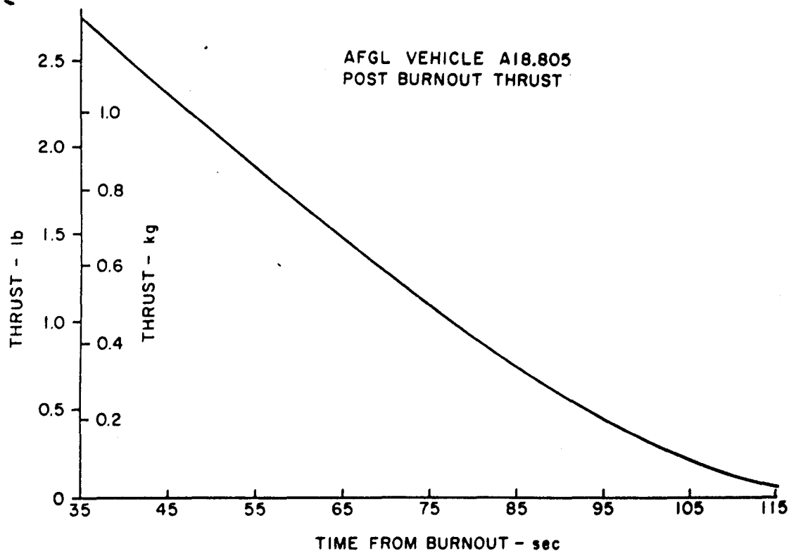
Figure 6. Thrust
