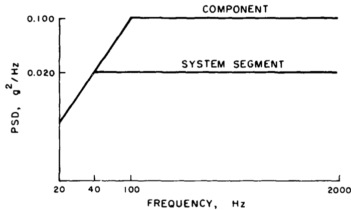
Figure A1. Aries Random Vibration Qualification Levels
