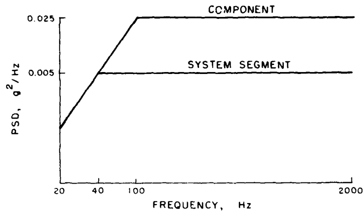
Figure A2. Arias Random Vibration Acceptance Level
