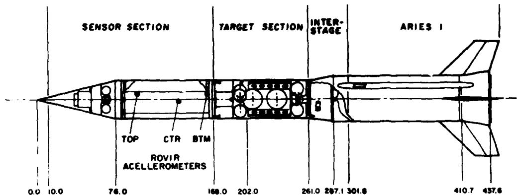
Figure 1. TEM-2 Vehicle
