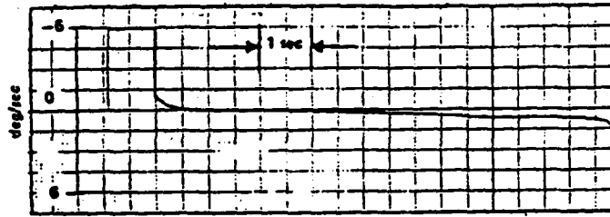
Fig. 9 Hybrid simulation pitch channel sample-and-hold output (gyro pitch rate).
