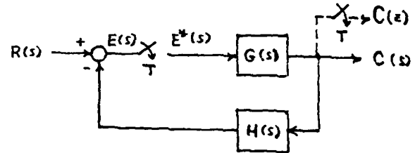
Figure. Closed-loop sampled-data system
