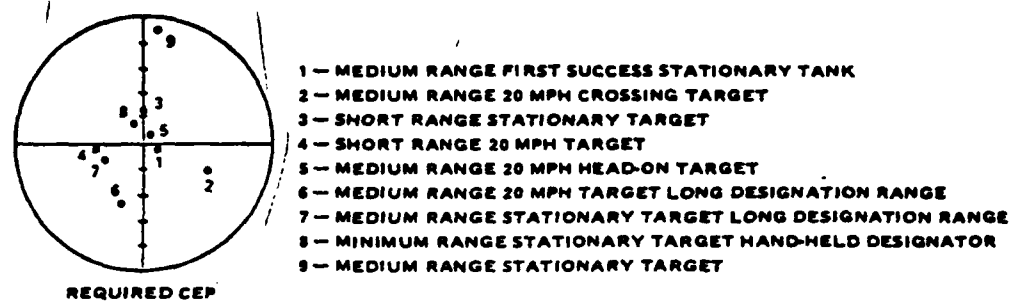
Fig. 17 Typical COPPERHEAD guidance and control performance.
