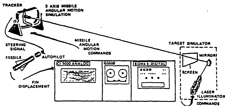
Fig. 8 Hardware-in-the-loop simulation.
