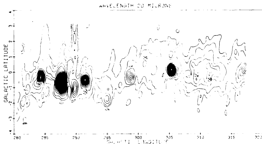
Figure 29. The 20- \mu m Map of the Galactic Equator Region Between 280^\circ and 320^\circ Longitude. The units for the contour levels are 10^{-11} \text{ W cm}^{-2} \mu\text{m}^{-1} \text{ sr}^{-1} . The numbers refer to associations with AFGL catalog sources. The wings at positive latitudes from 285^\circ to 290^\circ are due to baseline problems in the measurements.
