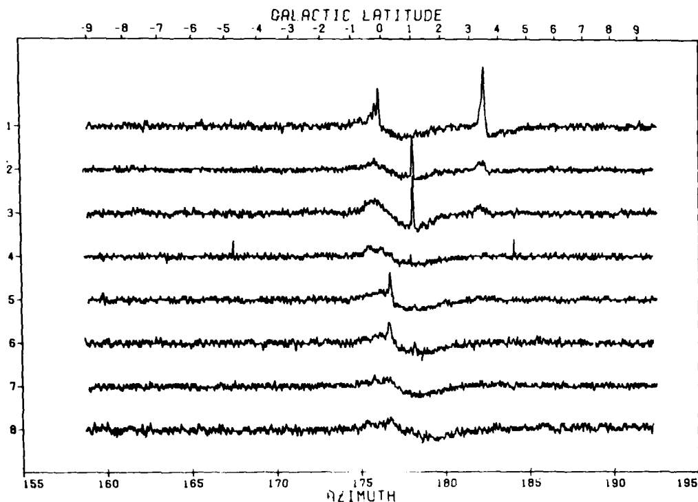
Figure 8. Uncompensated Output for a Galactic Plane Crossing. The longitude of the depicted region is about 30^\circ , AB Aql is the peak at b \sim 0.0 on channel one; W40 (Westerhout) is detected on channels 1 through 3 at b \sim 3.5
