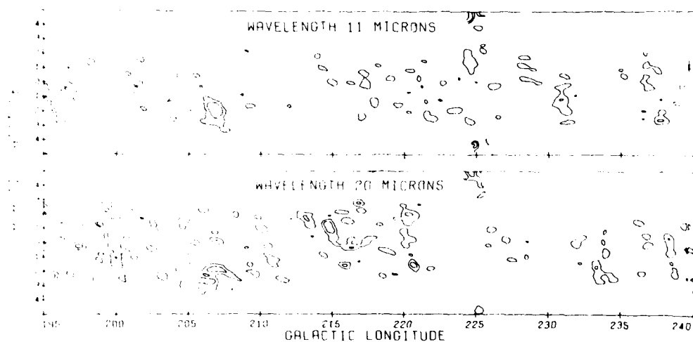
Figure 24. 11- and 20- \mu m Maps of the Galactic Plane from 195^{\circ} to 240^{\circ} Longitude. Contour levels are the same as defined in Figure 21. The resolution of these maps is approximately 0.7^{\circ} in latitude and 1.0^{\circ} in longitude
