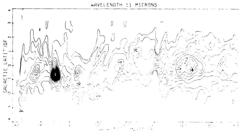
Figure 28. 11- \mu m Contour Map Along the Galactic Plane from 280^\circ to 320^\circ Longitude. This is an expanded version of the 11- \mu m map in Figure 27. The contour levels are in units of 10^{-11} \text{ W cm}^{-2} \mu\text{m}^{-1} \text{ sr}^{-1} . The AFGL source numbers of those sources associated with prominent extended objects in the map are also shown. Inadequate baseline correction produced the "pinching" of the contour around AFGL 4163, l \sim 305^\circ .
