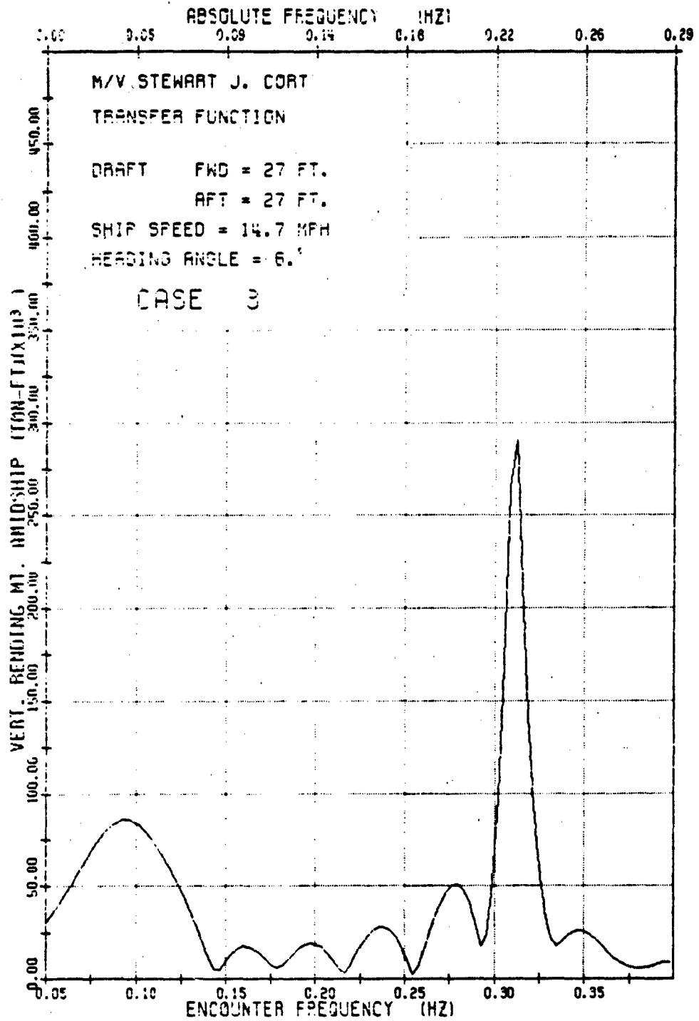
Fig. B3 - Transfer function, Case 3
