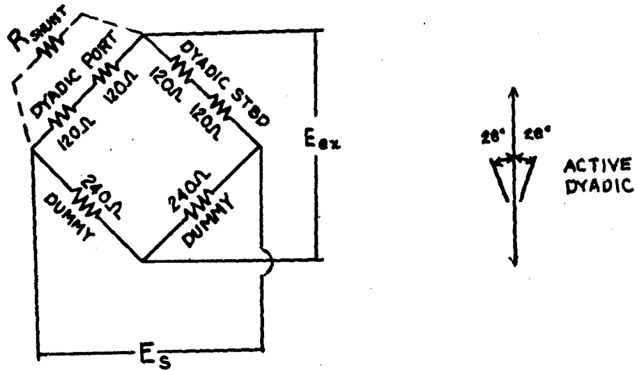
Figure A1 - Lateral and Main Deck Bending Bridge Configurations
