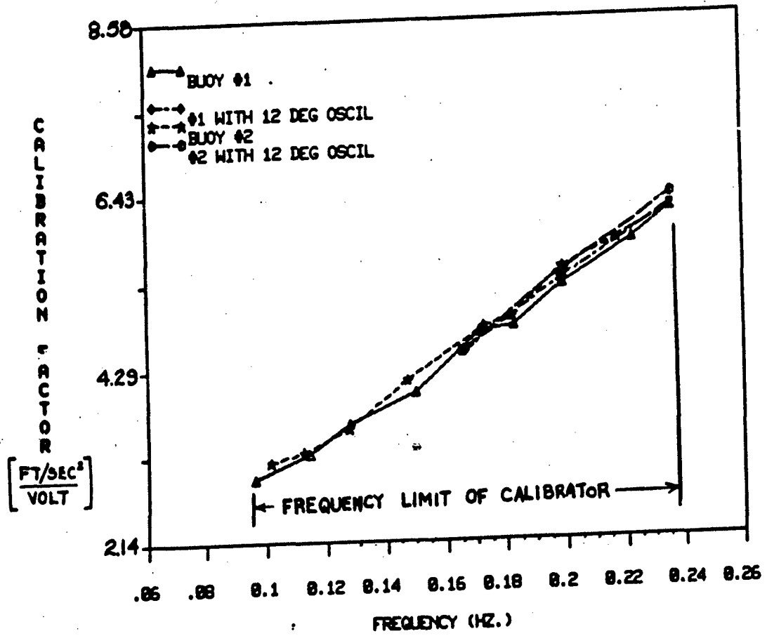
Figure A7 - Wave Rider Buoy Acceleration/Voltage Sensitivity
