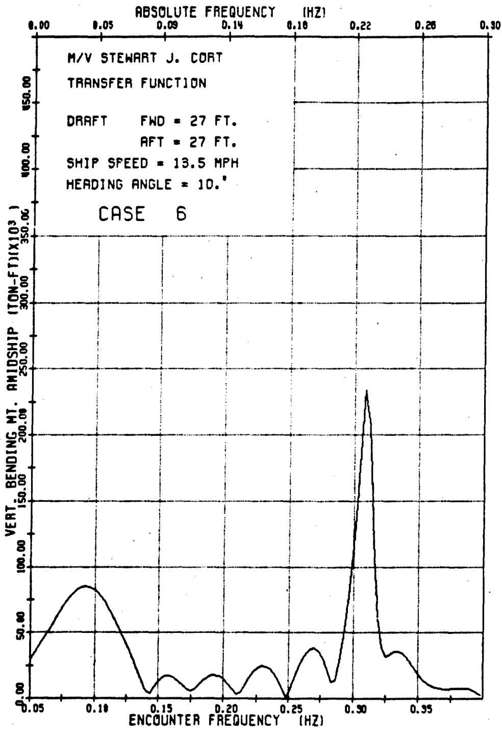
Fig. B6 - Transfer function, Case 6
