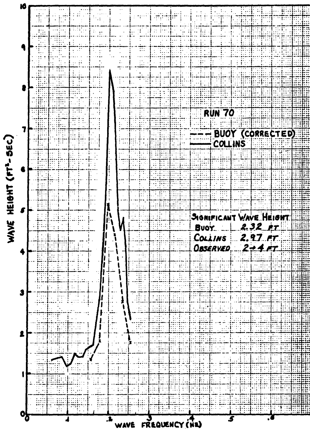
Figure 32 - Comparison of Wave Height Spectra Calculated from Collins Radar and Wave Rider Buoy for Run 70
