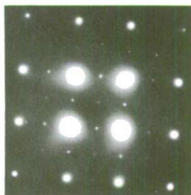
[001] ZONE AXIS
