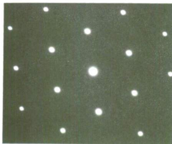
[011] ZONE AXIS
