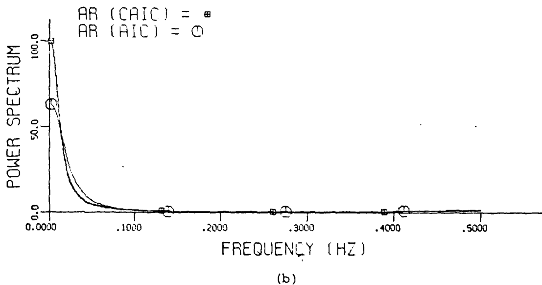
FIGURE III.1 Power spectrum of x_t = .4x_{t-1} + .5x_{t-2} + u_t .
