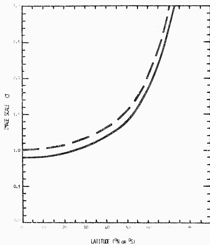
Figure 2.10. The latitudinal variation of image scale \sigma for Mercator projections true at 22.5^\circ\text{N}/22.5^\circ\text{S} (solid line) and 0^\circ (dashed line). The image scale as a function of latitude is symmetric about the Equator.
