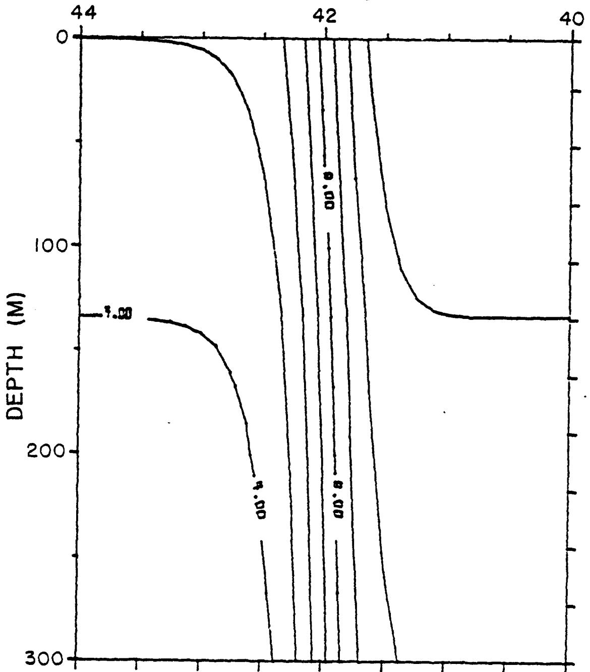
Figure 1. Initial position of the: a) temperature, and b) salinity fronts, in the (y, z) plane.
