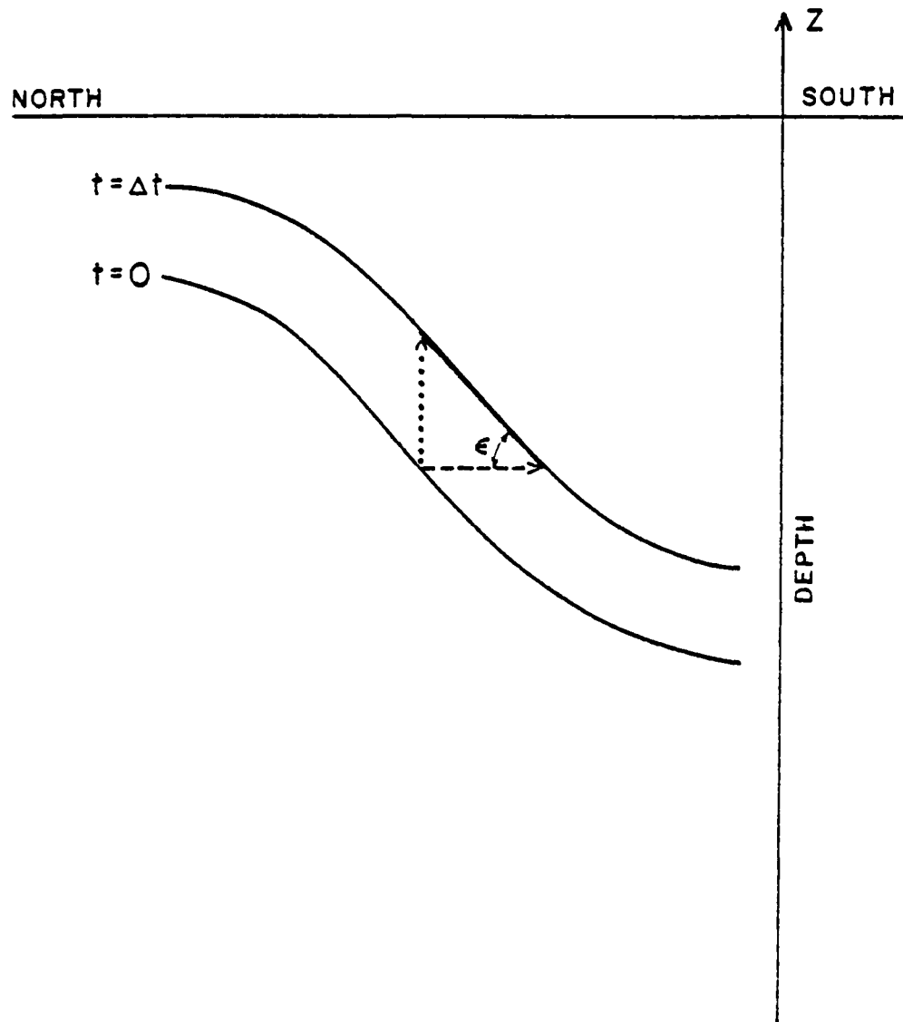
Figure 6. Relative positions of the first interface, represented by a solid line, near the front in the (y, z) plane at times t = \Delta t and t = 0 . The dotted line represents the vertical motion of the first interface, while the dashed line represents the southern motion of this same interface.
