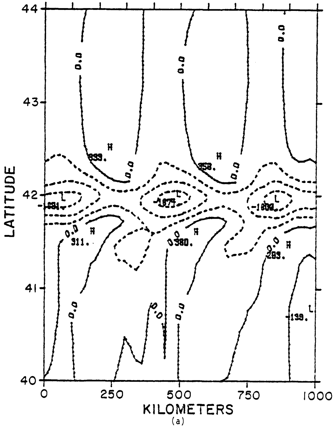
Figure 10. Isoanomalies of the height field a) for the first; b) the second; c) the third; and d) for the fourth layers, for the case of the cyclone travelling from west to east after 10 days.
