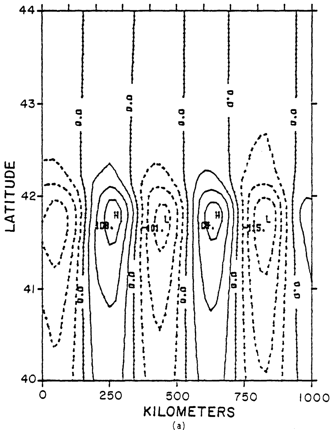
Figure 5. a) Isoanomalies of the zonal velocity field, u ; b) the meridional field, v ; c) the height field of the top layer for the cyclone travelling from west to east, after 7 days.
