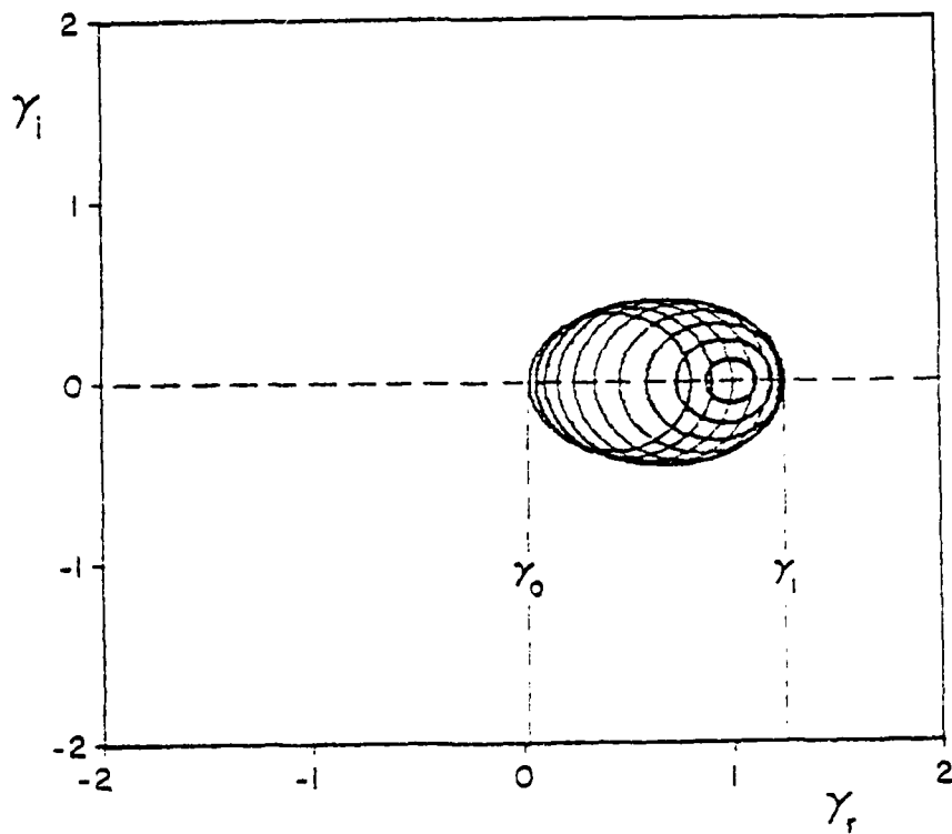
Figure 18. Circumference of equation |\gamma_r - u|^2 + \gamma_i^2 = \rho^2 in the complex \gamma plane for |u| \leq 1 .
