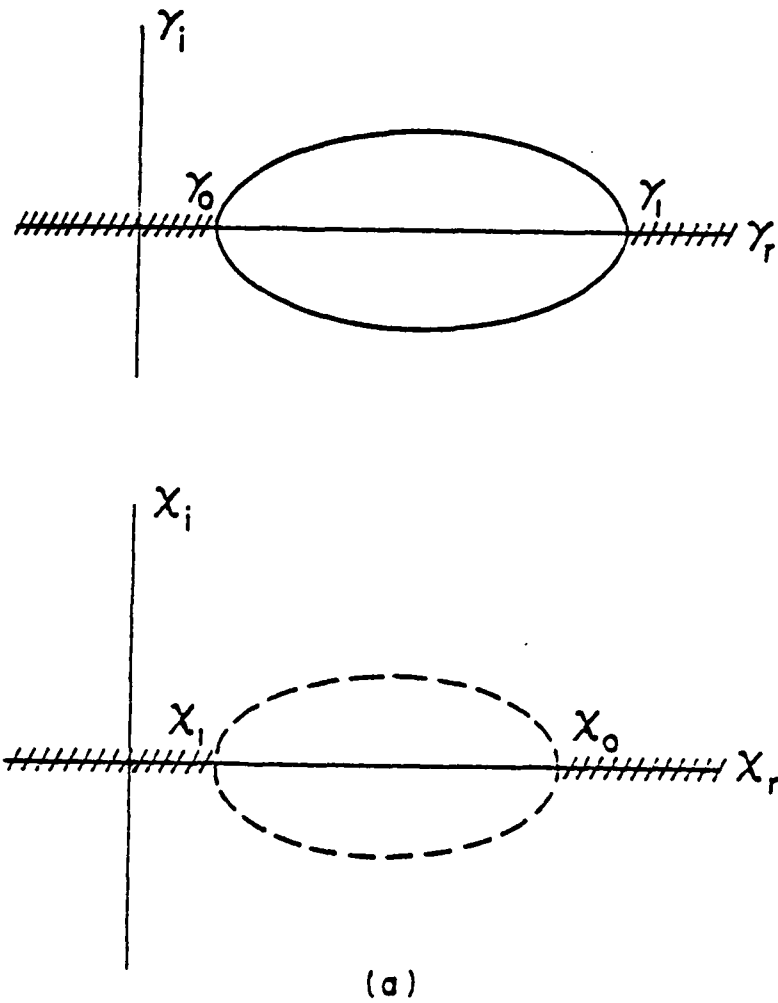
Figure 19. Region of stability in the x complex plane whenever a) \gamma_0 and \gamma_1 are positive, b) \gamma_0 and \gamma_1 are negative, c) \gamma_0 is negative and \gamma_1 is positive.
