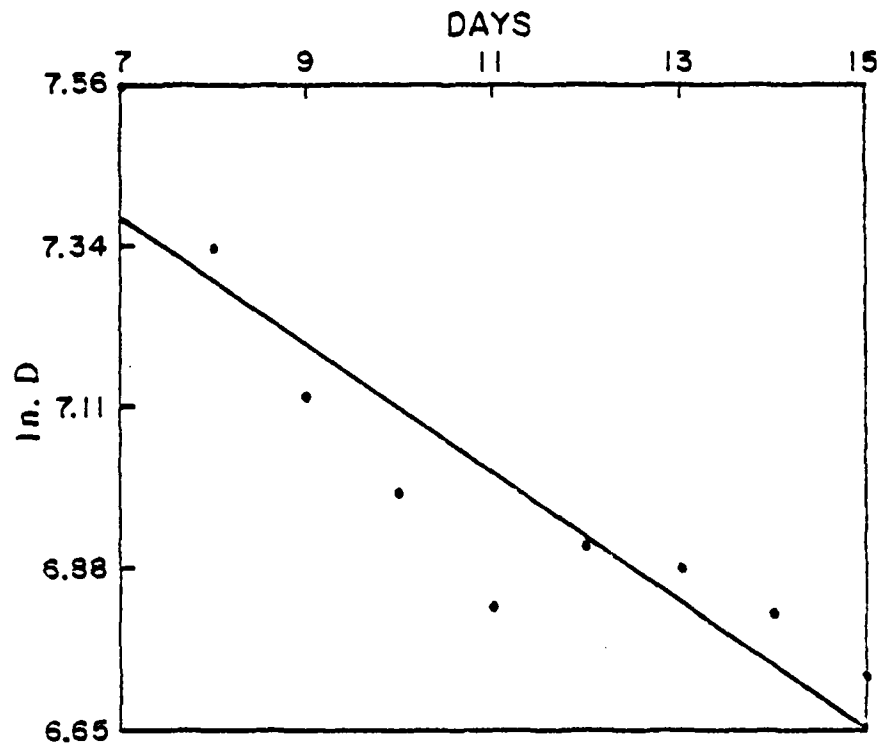
Figure 9. Decay in time of the amplitude of the vertical oscillation induced at the lee of the cyclone's track. While the dot points represent the original values of \ln D (see text), the solid line represents the curve obtained by using the least square method in (83).
