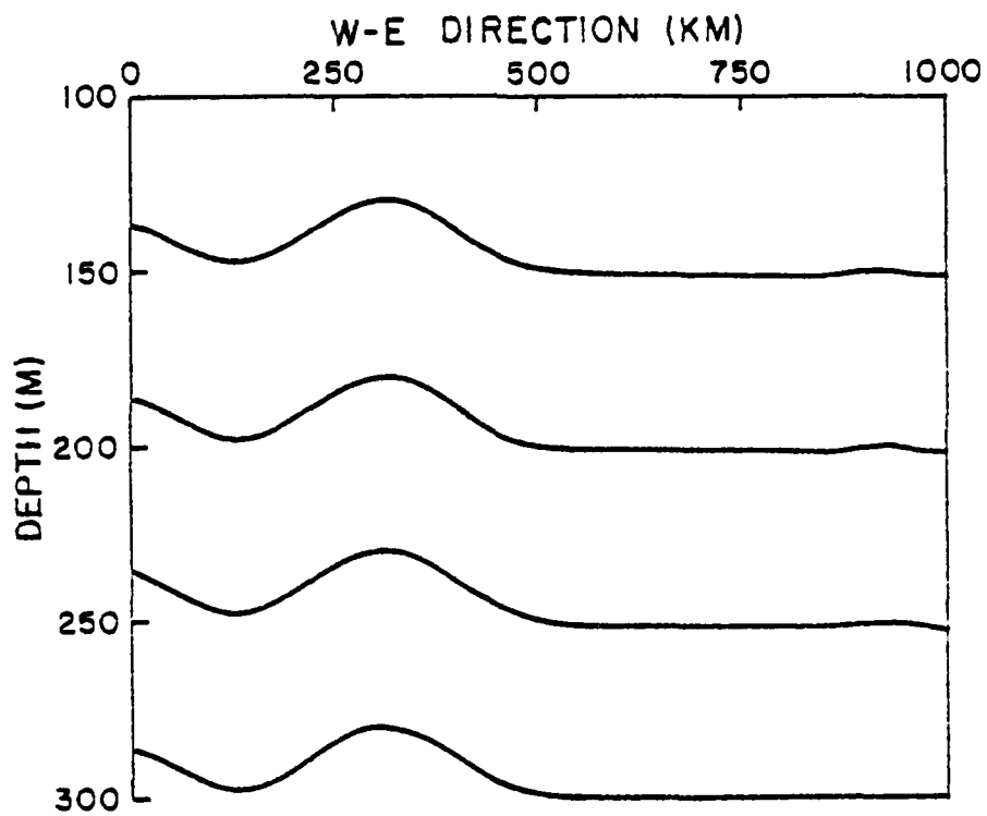
Figure 7. Cross section of the subarctic front in the (x, z) plane for the first cyclonic case after 5 days.
