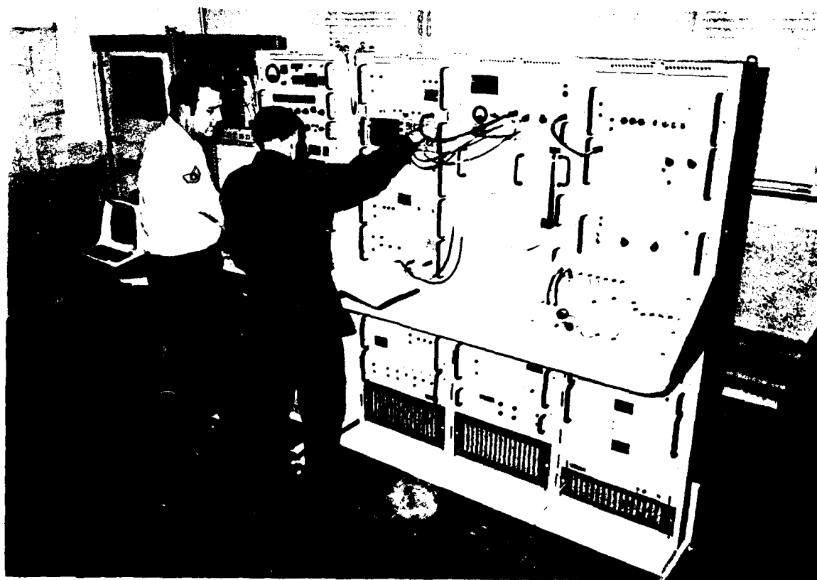
Burtek Flat Panel Simulation Of F-111D 6883 Flight Converter Test Station
