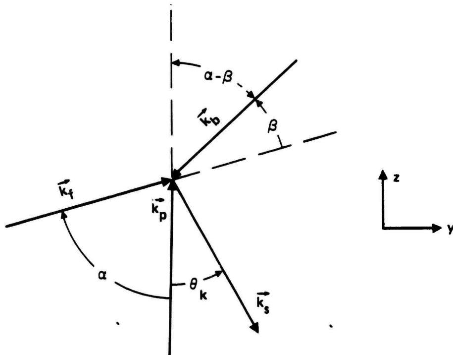
Figure 4-7. Generalized coplanar k vector geometry with pump-to-pump offset.
