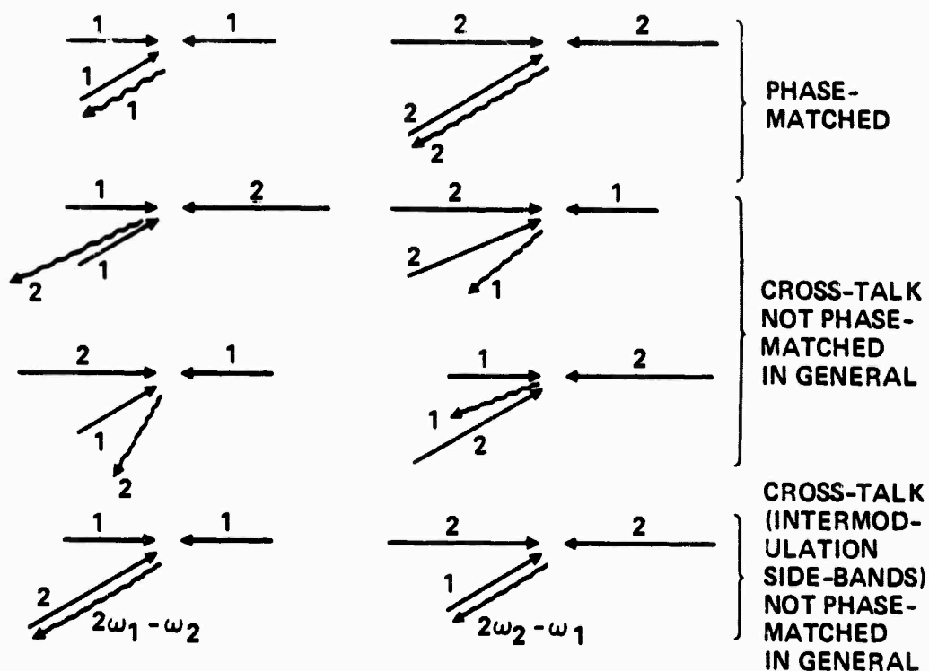
Figure 4-25. Classification of signal products in a four-wave mixer output when operating with 2-line pumps and probes.
