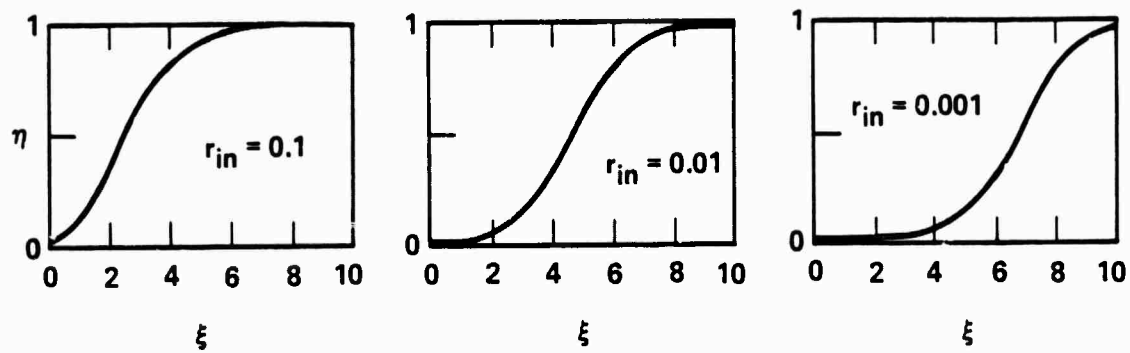
Figure 7-4. Efficiency \eta as a function of \xi = \gamma\eta_T vt .
