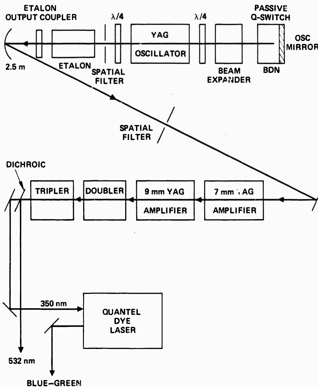
Figure 5-1. Quantel Yag-dye laser system.
