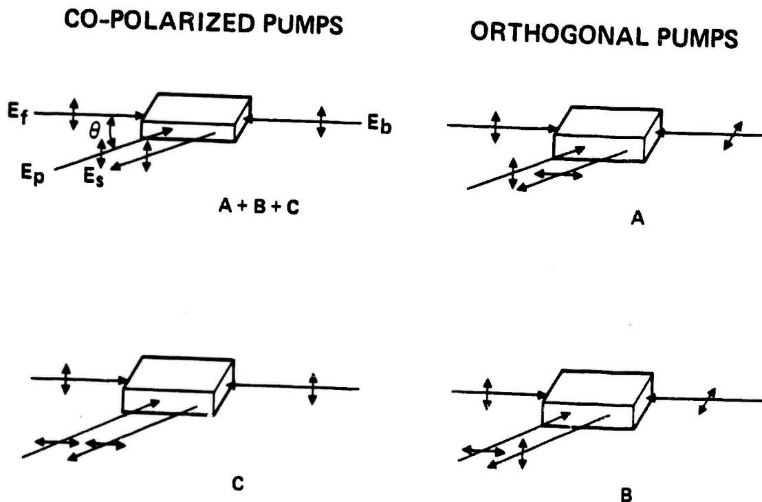
Figure 2-4. Polarization Options in DFWM (isotropic media).
