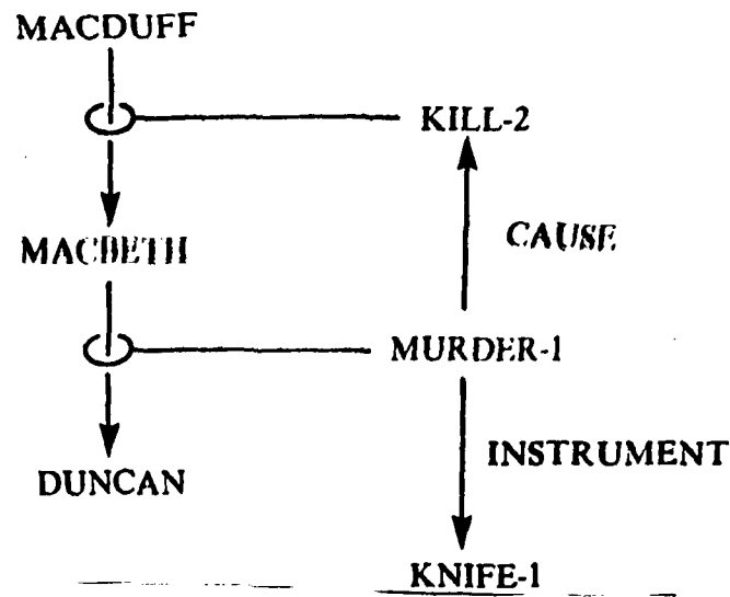
Figure 1: Supplementary description nodes MURDER-1 and KILL-2 carry case-like information supplementing the actor and object.
