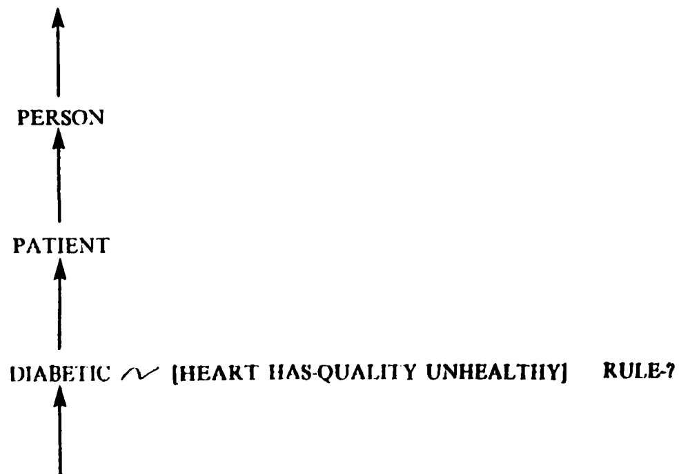
Figure 9: The rule for unhealthy hearts is stored under DIABETIC since the unhealthy heart used to construct the rule was part of a diabetic.
