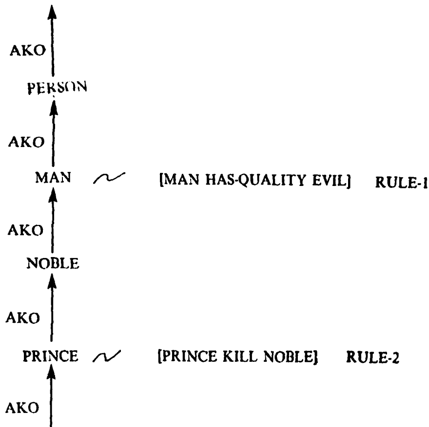
Figure 7: A rule is stored according to the class of the actor involved in the then part of the rule. Further indexing is done using the relation and the class of the object.
