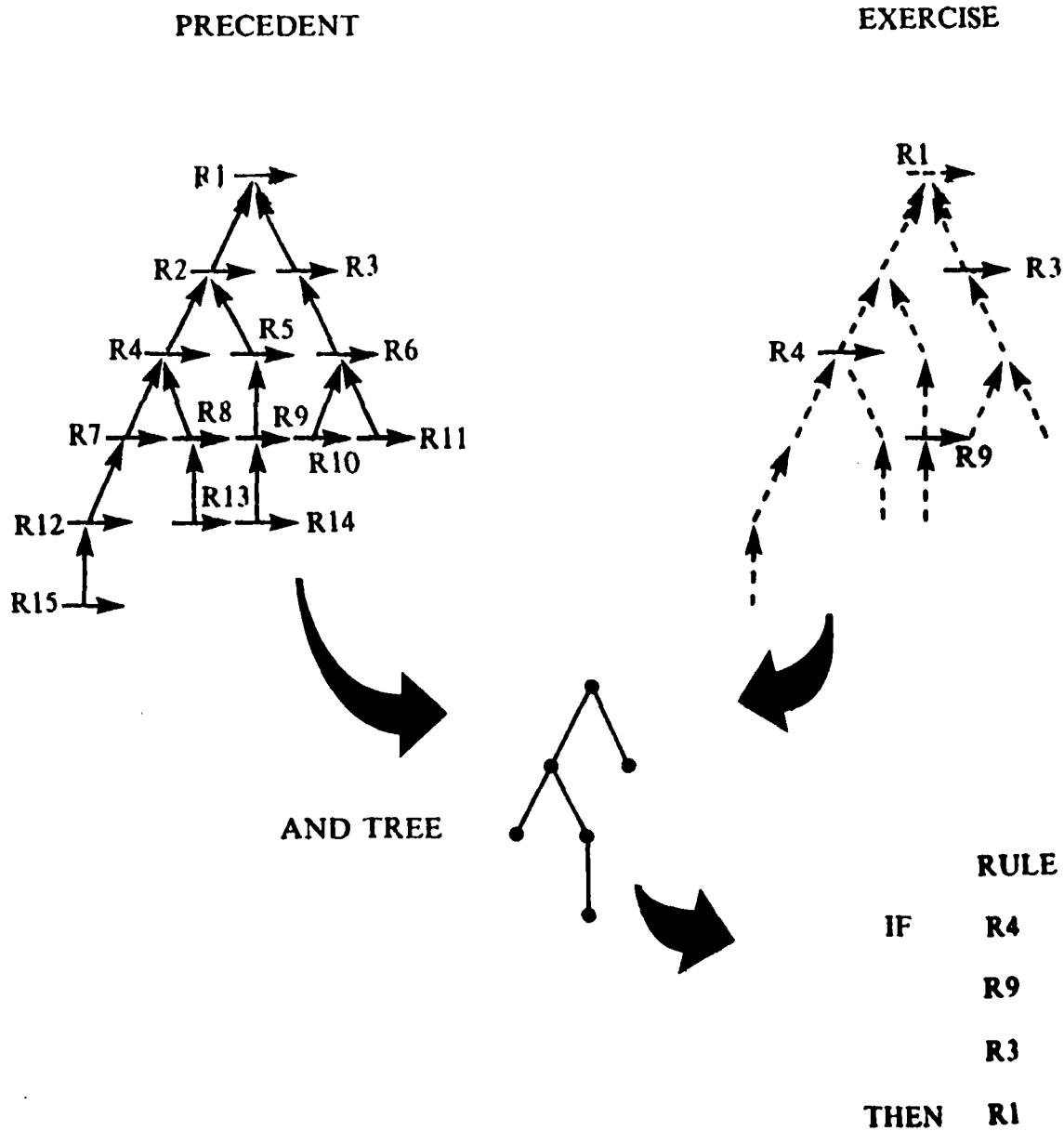
Figure 6: The rule synthesis procedure works because the precedent and the exercise determine an AND tree, from which the rule is made. The tips go into the if part of the rule and the root into the then part.
