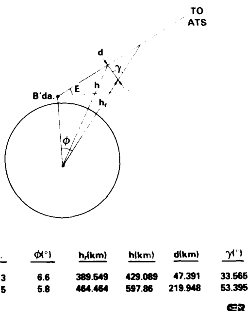
Fig. 10 — Determination of the orientation of the raypaths with respect to the rocket at closest approach
