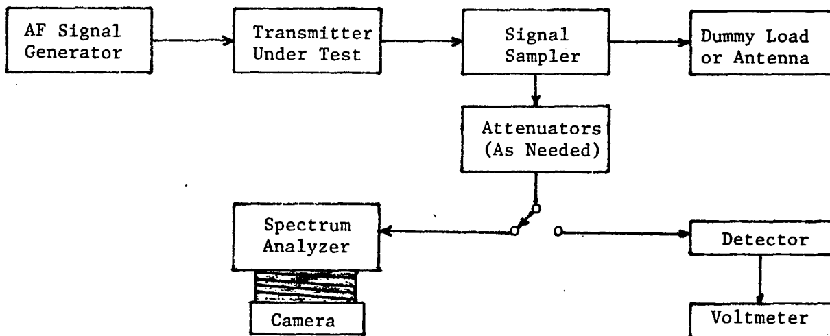
Figure 6 - Block Diagram of Carrier Noise Level Measurements
